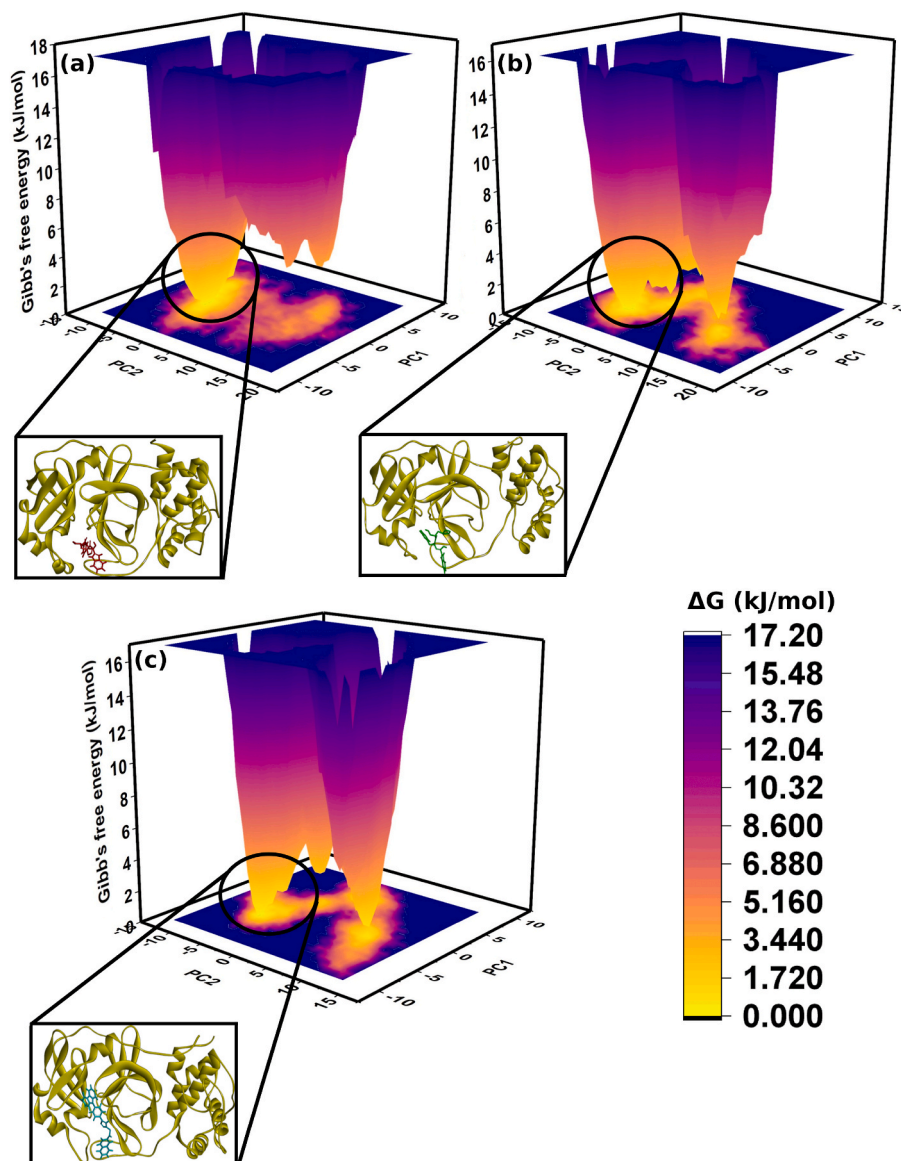
Fig. 5. Free energy landscape of M^{pro} as a function of first two principal components PC1 and PC2 (a) 11a, (b) 11b, and (c) 3h.
