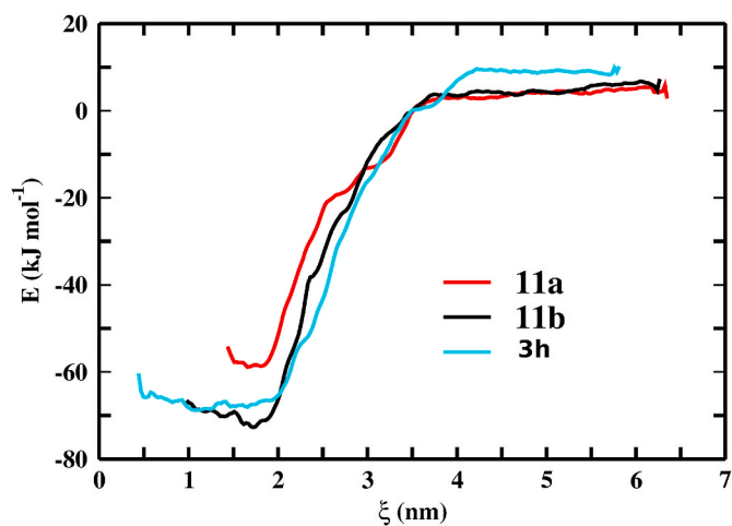
Fig. 6. Potential of mean force (PMF) curves obtained after umbrella sampling for the co-crystallized and the best selected compound in complex with M^{pro} SARS-CoV-2.
