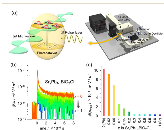
Fig. 8 (a) Schematic image of TRMC measurement. (b) TRMC transients of \text{Sr}_x\text{Pb}_{1-x}\text{BiO}_2\text{Cl} (orange for x = 0 to blue for x = 1 ). (c) \varphi\Sigma\mu_{\text{max}} values with respect to x for \lambda_{\text{ex}} = 266 nm and I_0 = 6.8 \times 10^{15} photons \text{cm}^{-2} per pulse. (b and c) Adapted with permission from ref. 35 Copyright 2020, American Chemical Society.
