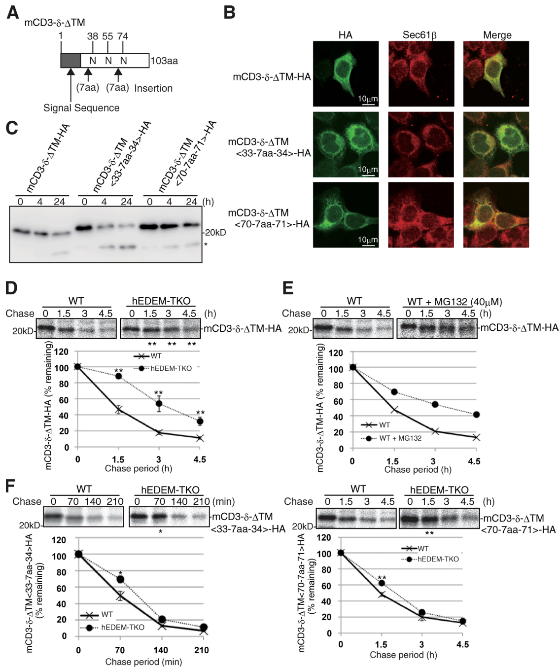
Figure 4. Effect of EDEM-TKO on mCD3- \delta - \Delta TM degradation. (A) Schematic structures of WT and two insertion mutants of mCD3- \delta - \Delta TM. (B) Immunofluorescence of HCT116 cells expressing transfected WT or insertion mutant of mCD3- \delta - \Delta TM using anti-HA. (C) PNGase sensitivity assay of WT and two insertion mutants of mCD3- \delta - \Delta TM expressed in HCT116 cells by transfection (immunoblotting with anti-HA). The asterisk denotes partially deglycosylated mCD3- \delta - \Delta TM. (D) Pulse-chase to determine the degradation rate of transfected WT mCD3- \delta - \Delta TM in WT and hEDEM-TKO cells using anti-HA ( n = 3 ). (E) Pulse-chase to determine the degradation rate of transfected WT mCD3- \delta - \Delta TM in WT cells and those treated with 40 \mu M MG132 using anti-HA. This experiment was completed once. (F) Pulse-chase to determine the degradation rate of transfected insertion mutants of mCD3- \delta - \Delta TM in WT and hEDEM-TKO cells using anti-HA ( n = 3 ). (D–F) Means \pm SD are shown. (D and F) *, P < 0.05 ; **, P < 0.01 .
