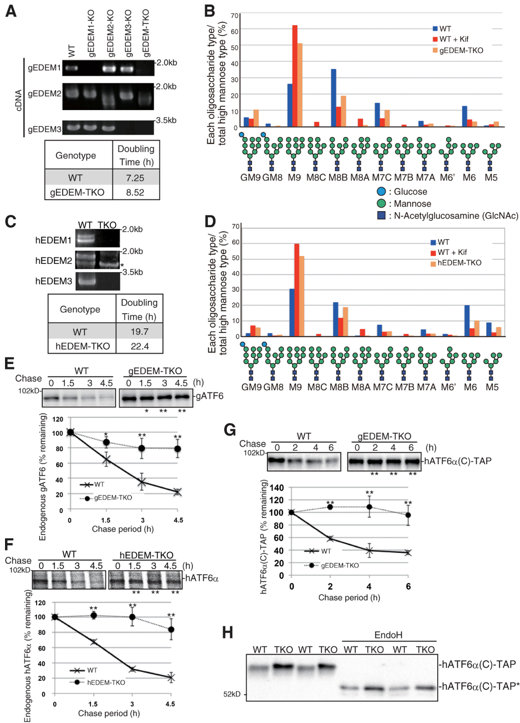
Figure 1. Effect of EDEM-TKO on N-glycan profiles and ATF6 \alpha degradation. (A) RT-PCR to amplify cDNA corresponding to gEDEM1/2/3 mRNA in DT40 cells of various genotypes and doubling times of WT and gEDEM-TKO cells. (B) Isomer composition of N-glycans prepared from total cellular glycoproteins of WT, WT treated with kifunensine (Kif, 10 \mu g/ml, 6 h), and gEDEM-TKO cells. This experiment was completed once. (C) RT-PCR to amplify cDNA corresponding to hEDEM1/2/3 mRNA in WT and hEDEM-TKO cells and their doubling times. The asterisk denotes a nonspecific band. (D) Isomer composition of N-glycans prepared from total cellular glycoproteins of WT, WT treated with kifunensine (10 \mu g/ml, 12 h), and hEDEM-TKO cells. This experiment was completed once. (E) Cycloheximide chase to determine the degradation rate of endogenous gATF6 (only one ATF6 gene in chicken genome) in WT and gEDEM-TKO cells using anti-gATF6 ( n = 3 ). (F) Pulse-chase to determine the degradation rate of endogenous hATF6 \alpha in WT and hEDEM-TKO cells using anti-hATF6 \alpha ( n = 3 ). (G) Cycloheximide chase to determine the degradation rate of transfected hATF6 \alpha (C)-TAP in WT and gEDEM-TKO cells using anti-c-myc ( n = 3 ). (E–G) Means \pm SD are shown. *, P < 0.05 ; **, P < 0.01 . (H) Immunoblotting of cell lysates prepared from WT and gEDEM-TKO cells expressing transfected hATF6 \alpha (C)-TAP with or without EndoH treatment using anti-c-myc. hATF6 \alpha (C)-TAP* denotes the nonglycosylated hATF6 \alpha (C)-TAP.
