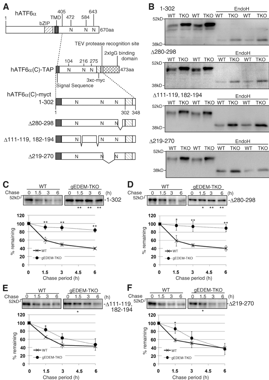
Figure 3. Effect of EDEM-TKO on hATF6 \alpha (C)-myct degradation. (A) Schematic structures of hATF6 \alpha , hATF6 \alpha (C)-TAP, hATF6 \alpha (C)-myct, and its three deletion mutants. bZIP and TMD denote basic leucine zipper and transmembrane domains, respectively. N indicates a potential glycosylation site. Both the amino acids 111–119 and 182–194 are expected to form an \alpha -helix. (B) Immunoblotting of cell lysates prepared from WT and gEDEM-TKO cells expressing one of the four hATF6 \alpha (C) derivatives by transfection with or without EndoH treatment using anti-c-myc. (C–F) Cycloheximide chase of WT and gEDEM-TKO cells expressing one of the four hATF6 \alpha (C) derivatives by transfection using anti-c-myc ( n = 3 ). Means \pm SD are shown. *, P < 0.05 ; **, P < 0.01 .
