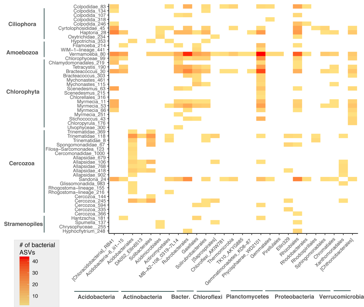
Fig. 4. Many protistan and bacterial taxa are highly correlated. Pairwise correlation heatmap of co-occurrences between protistan and prokaryotic ASVs (those found at >10\% of sites). The bacterial ASVs (x axis) are collapsed by order-level taxonomy for readability—the heatmap color indicates the number of bacterial ASVs that were correlated with a particular protistan ASV (y axis).
