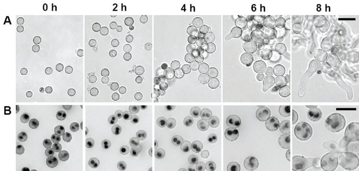
Fig. 1. Germination of A. niger conidia as observed by bright-field (A) and fluorescence microscopy ( \lambda = 450\text{--}490 nm, FT510, LP520) (B). In (B) A. niger RB#9.5 was used. This strain expresses a gene encoding a fusion between sGFP and the histone H2B. The fusion protein is targeted to the nucleus. Bar represents 10 \mu\text{m} (A) and 5 \mu\text{m} (B).
