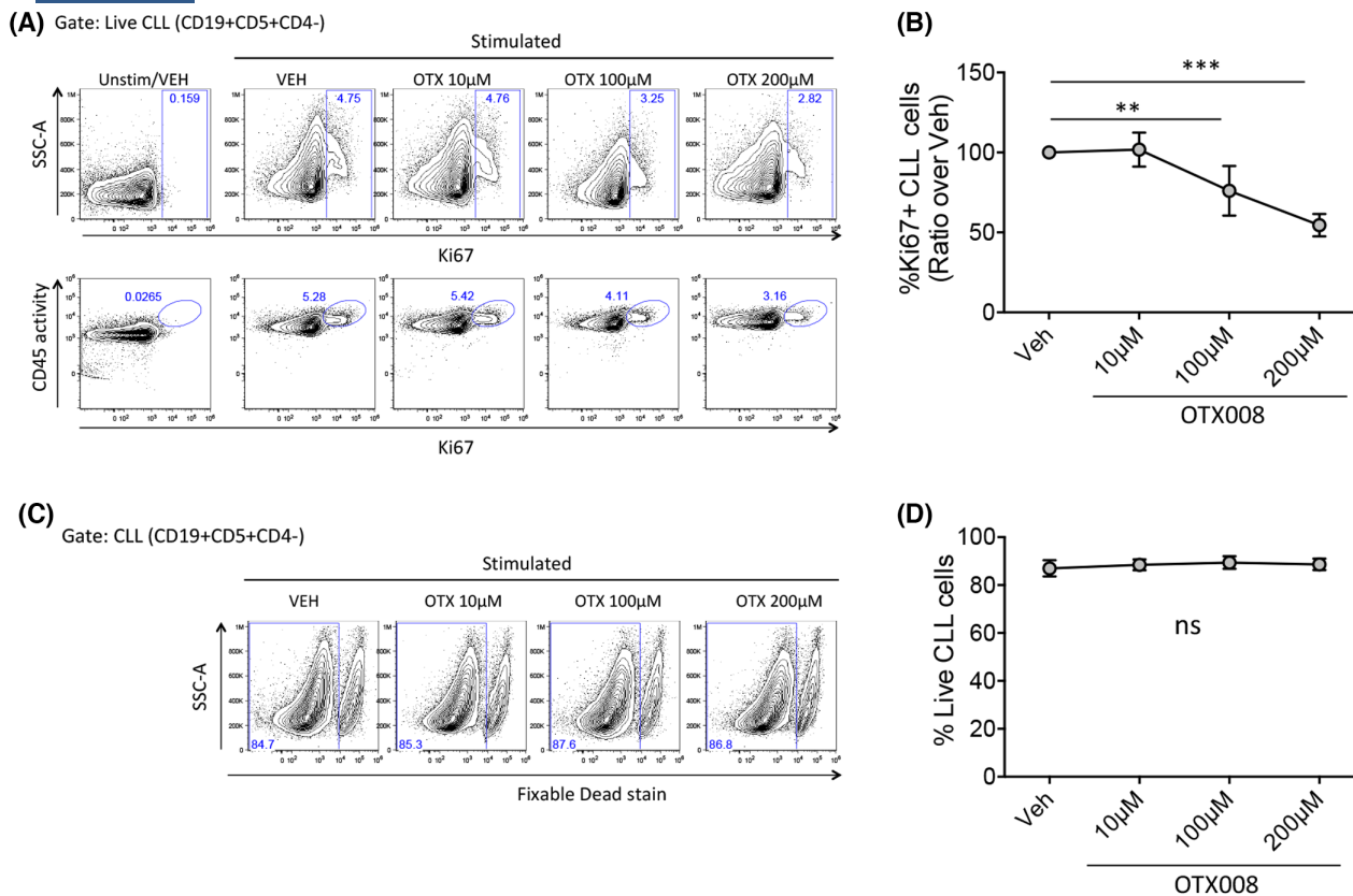
FIGURE 6 Direct effect of OTX008 on CLL cell proliferation. (A) Representative flow cytometry dot plots reveal a reduction in isolated CLL cell proliferation with OTX008 treatment (upper panels) and a concomitant reduction in the Ki67 + /CD45 activity + population (lower panels). (B) Graph shows means \pm SD of %Ki67 + CLL cells (ratio over Veh). (C) OTX008 did not induce cell death in isolated CLL cells. (D) Graph shows means \pm SD of %live CLL cells. Statistical significance was defined by repeated-measures one-way ANOVA with Dunn's correction. Data are representative of eight CLL patient samples. ** p \leq 0.01 ; *** p \leq 0.001 . ANOVA, analysis of variance; CLL, chronic lymphocytic leukaemia. [Colour figure can be viewed at wileyonlinelibrary.com ]
