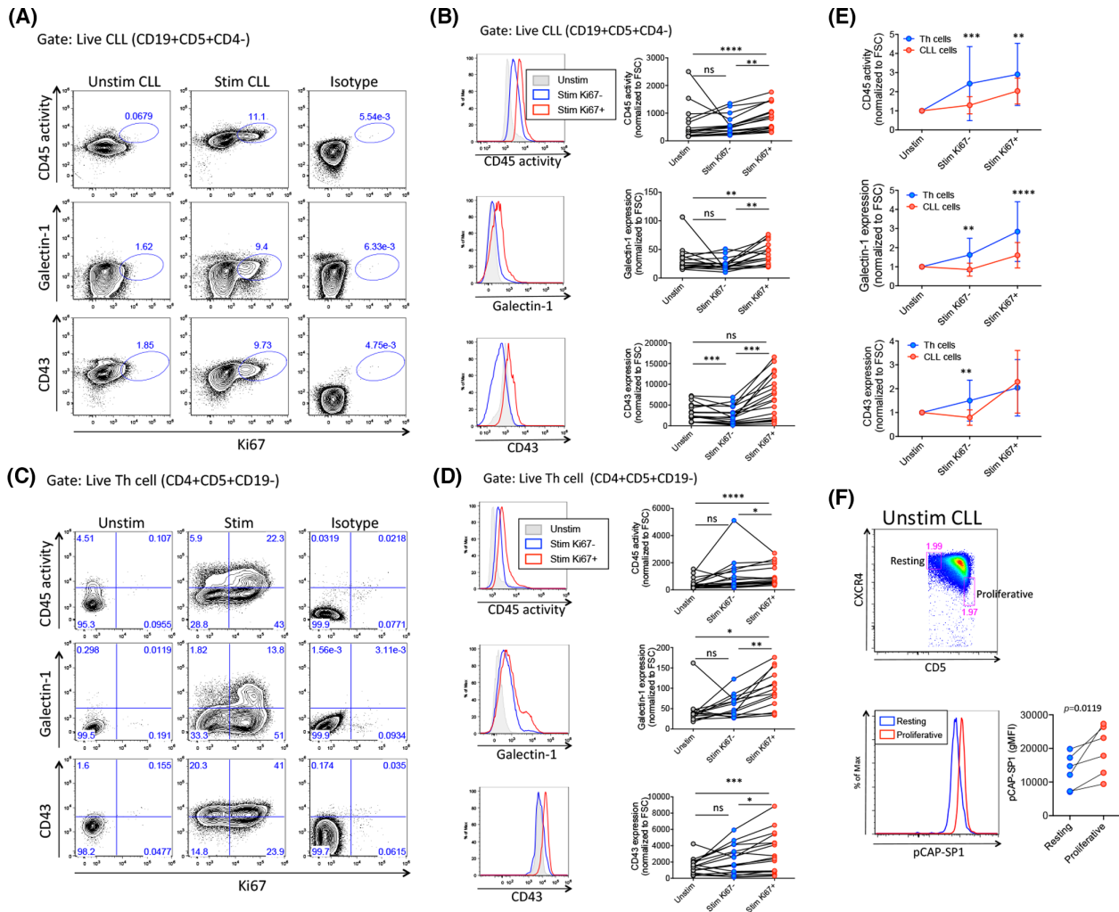
FIGURE 4 Proliferating CLL and Th cells have increased CD45 activity, galectin-1, and CD43 expression. Representative flow cytometry dot plots showing proliferation ( Ki67^+ ) associated with increasing CD45 activity (upper panels), galectin-1 surface staining (middle panels), and CD43 surface expression (lower panels) in CLL cells (A) or Th cells (C). Graphs show paired individual values (normalised to size) from patients for gMFI CD45 activity (upper panels), galectin-1 surface staining (middle panels), and CD43 surface expression (lower panels) in gated live CLL cells (B) and Th cells (D). (E) Galectin-1 was more robustly increased on proliferating Th cells versus proliferating CLL cells. (F) the proliferative ( CXCR4^{dim}CD5^{bright} ) CLL cell subpopulation in peripheral blood had higher CD45 activity in comparison to the non-proliferative, resting subpopulation ( CXCR4^{bright}CD5^{dim} ). Included is a representative flow cytometry dot plot and histogram. Graphs show means \pm SD. Statistical significance was defined by Friedman test with Dunn's correction (B upper and middle panels, D), repeated-measures one-way ANOVA with Sidak's correction (B lower panel), two-way ANOVA (E), or Student's paired t -test (F). Data are representative of 18 (A–E) and six (F) CLL patient samples. ** p \leq 0.01 ; *** p \leq 0.001 ; **** p \leq 0.0001 . ANOVA, analysis of variance; CLL, chronic lymphocytic leukaemia; gMFI, geometric mean of fluorescence intensity; Th, T-helper. [Colour figure can be viewed at wileyonlinelibrary.com ]
