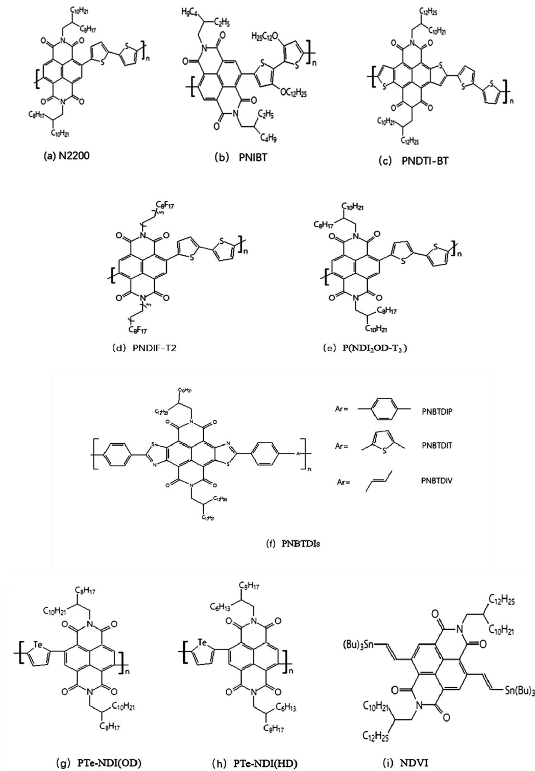
Fig. 1 Representative molecular structures (a–i) of naphthalene diimide based N-type polymer semiconductors.
