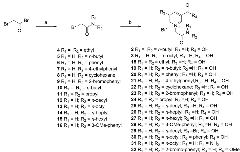
Figure 2. Synthesis of small-molecule NAADP analogues. Reagents and conditions: (a) R_1R_2NH , ether, ice-salt bath; (b) Nicotinic acid (or nicotinic acid derivative), DME, 60–70 °C, 16 h.
