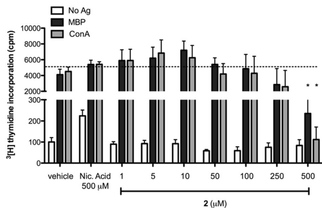
Figure 6. Inhibitory effect of 2 on antigen (MBP, black bars) and mitogen (ConA, grey bars) induced proliferation in T_{MBP} cells, as evaluated via [ ^3H ]-thymidine incorporation. White bars show basal proliferative levels of cells in absence of specific activation. Data are presented as mean \pm SEM of five independent experiments. Vehicle and nicotinic acid (500 \mu M) were used as internal controls. Two-way ANOVA test shows statistically relevant differences in proliferation upon incubation with high doses of 2 , when compared to vehicle (threshold dotted line); (*) p < 0.05 .
