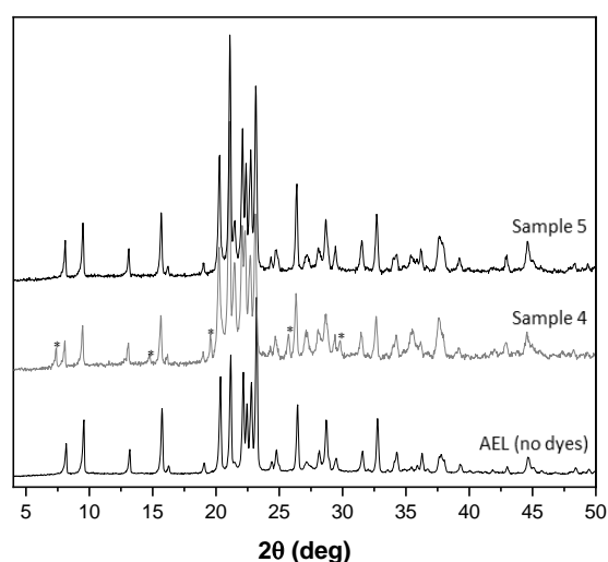
Figure A1. XRD patterns of AEL materials, without dyes ( bottom ), Sample 4 ( middle ), and Sample 5 ( top ); * indicates minor impurities of AFI material.
