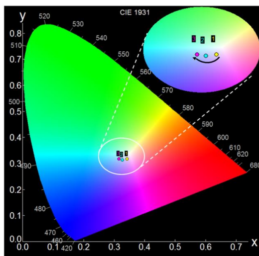
Figure A4. Changes in the CIE coordinates of Sample 4 at different times of intense UV irradiation ( \lambda_{exc} = 355 nm and an irradiance of 2.75 mW/cm 2 ): t = 0 (point 1); t = 1 h (point 2) and t = 6 h (point 3).
