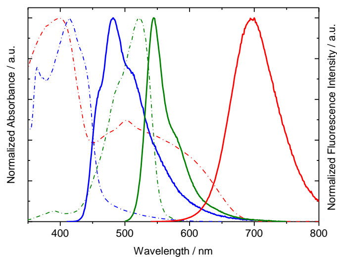
Figure 1. Normalized absorption spectra (dashed lines) and fluorescence spectra (solid lines) of MgAPO-11 samples containing a unique dye: AC/AEL (blue lines), PY/AEL (green lines), and LDS722/AEL (red lines).
