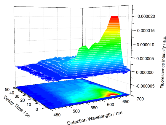
Figure A2. Time-resolved fluorescence emission spectra of Sample 4 recorded by fs fluorescence up-conversion in 50 ps time window ( \lambda_{exc} = 395 nm).
