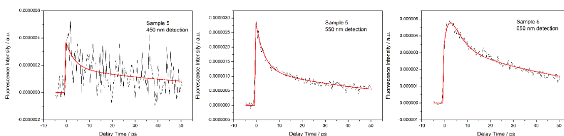
Figure 5. Decay traces recorded by fs fluorescence up-conversion for Sample 5 (3:1:2) at 450, 550, and 650 nm detection wavelength ( \lambda_{\text{exc}} = 395 nm).
