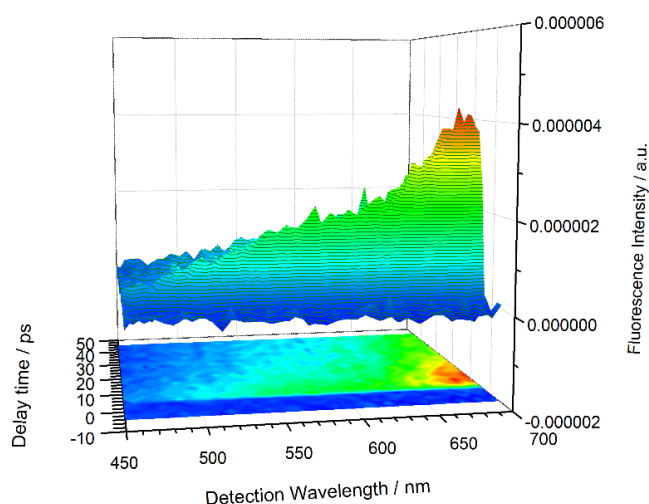
Figure A3. Time-resolved fluorescence emission spectra of Sample 5 recorded by fs fluorescence up-conversion in 50 ps time window ( \lambda_{exc} = 395 nm).
