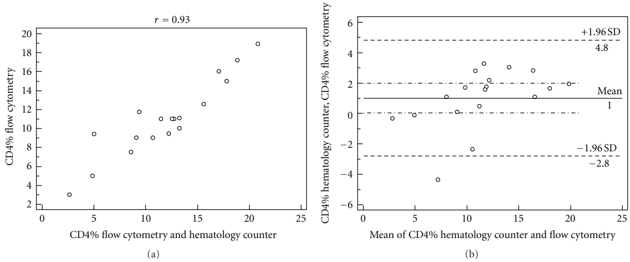
FIGURE 1: Correlation of percentage values of CD4+, P < 0.05 (a) and limits of agreement between the values estimated by Bland-Altman analysis (b) obtained by the hematology counter and the flow cytometer in the stratum of CD4 count < 200 cells/mL.
