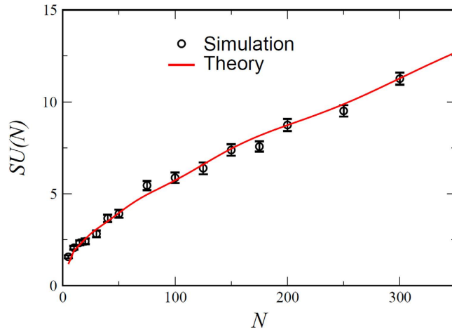
Figure 3. The number of SU states as a function of N for the asymmetric zero-infinity model (note the linear scale, in contrast to Fig. 2). Results were obtained from an average over simulations of random networks with \tilde{p} = 0.5 , N running from 5 to 300. Points correspond to the number of SU states in a single realization, full line is the exact sum over S of (4). The asymptotic relationship (5) converges to this sum very slowly, see SI section II.
