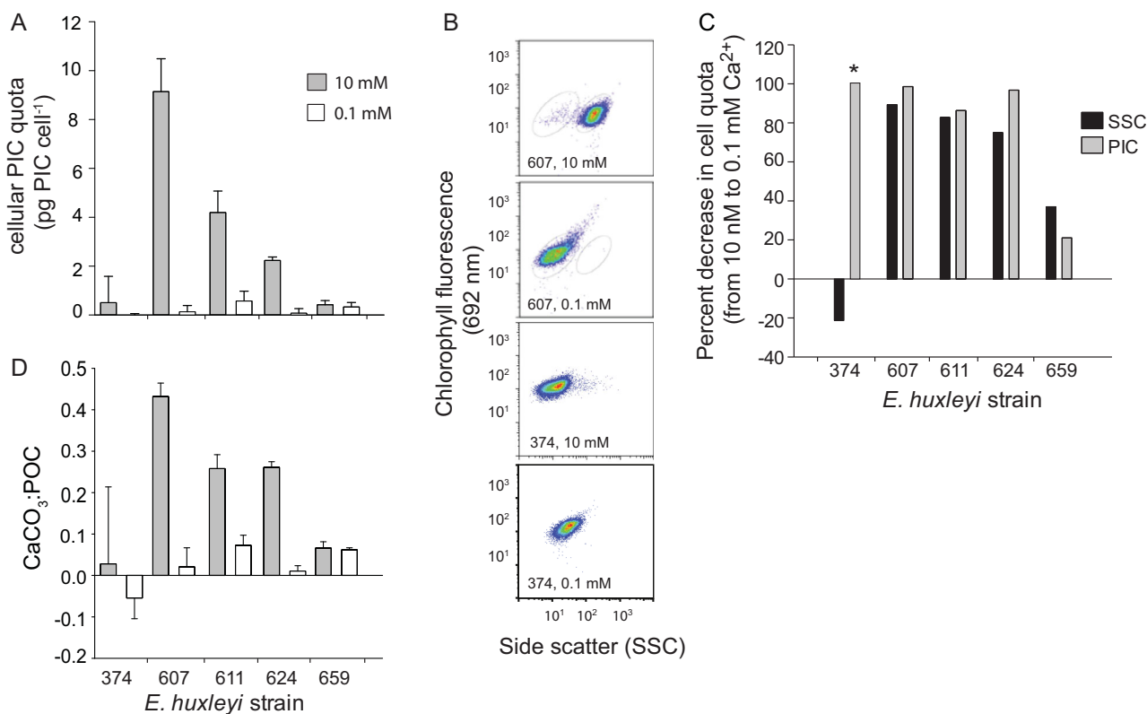
Fig. 3. Calcification state of various E. huxleyi strains grown in defined ESAW media at different \text{Ca}^{2+} concentrations. (A) Cellular PIC quota for strains grown with either 0.1 mM or 10 mM \text{Ca}^{2+} concentrations. Error bars represent the standard error ( \text{SD}/\sqrt{n} ) among triplicate measurements for one experiment; host–virus dynamics shown were representative of experiments ( n = 3 ) performed on different dates. (B) Representative flow cytometry plot showing the SSC and chlorophyll (692 nm) signals for DHB607 grown in 10 mM or 0.1 mM \text{Ca}^{2+} compared to canonical naked strain CCMP374 grown in 10 mM \text{Ca}^{2+} . Note the prominent shift to a lower SSC for DHB607 cells grown in 0.1 mM, matching that of the low SSC for CCMP374. (C) Percentage (%) decrease in both the mean cellular PIC quota and geometric mean of SSC for cells grown in 10 mM \text{Ca}^{2+} compared to those grown in 0.1 mM \text{Ca}^{2+} (asterisk for strain CCMP374 denotes that the % decrease in PIC derives from a 0 pg PIC cell -1 at 0.1 mM \text{Ca}^{2+} ). (D) \text{CaCO}_3 :POC ratios derived from the data in panel (A). We noted that growth in the ESAW artificial seawater medium at 10 mM \text{Ca}^{2+} did generally lower the total calcification state for all DHB strains compared to cells grown in f/2-Si media (Figs 1A and 3A), likely due to the presence of additional factors in seawater-based media that are required for maximum calcification. Nonetheless, these strains clearly calcified in ESAW media, maintained similar growth rates, and possessed similar cellular chlorophyll signatures, indicative of healthy cells. SEM images confirmed that there was plenty of calcite production in culture under these conditions, with the formation of fully formed coccospheres and detached coccoliths (Supporting Information Fig. S2).
