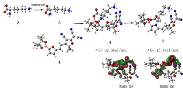
Fig. 5 Density functional theory (DFT) calculations on the reaction of DFC and L-Lys.
