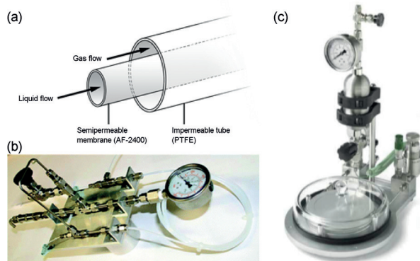
Figure 4. a) Annular, tube-in-tube fluid-flow regions. The semipermeable membrane tubing is placed inside an impermeable PTFE outer layer. b) Prototype reactor used to facilitate gas–liquid reactions. [27] Reproduced with permission from The Royal Society of Chemistry. c) The Gastropod reactor from Cambridge Reactor Design, a commercially available unit that was developed from this study. [29]
