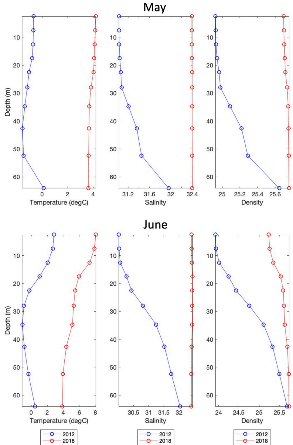
Fig 11. Vertical sections of temperature, salinity, and density. Vertical sections of temperature ( ^{\circ} C), salinity, and density ( \sigma ) during May (upper) and June (lower) for 2012 (blue) and 2018 (red) from RASM at 60.5 ^{\circ} N, 175 ^{\circ} W (location shown as a small black circle in Fig 10).
