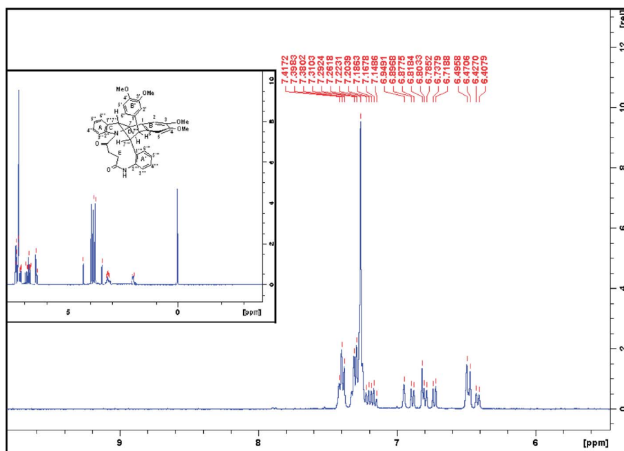
Fig. 3 ^1\text{H} NMR ( \text{CDCl}_3 , 400 MHz) spectrum of compound (73) Scheme 17.
