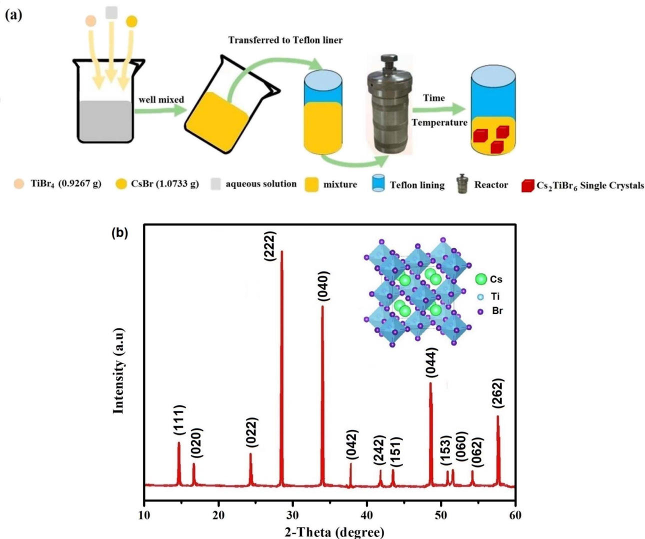
Fig. 1 (a) Schematic illustration of the slow cooling method to obtain Cs 2 TiBr 6 SCs. (b) Powder X-ray diffraction pattern of Cs 2 TiBr 6 obtained at ambient temperature within the 2θ range of 10–60°. The inset displays the arrangement of Cs 2 TiBr 6 in the crystal lattice.
