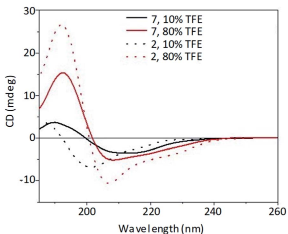
Fig. 3 Far-UV CD spectra of peptide 2 (53 \mu M, dot line) and POM-(peptide) 2 7 (26.5 \mu M, solid line) at different TFE : water percentage (10% black line, 80% red line).
