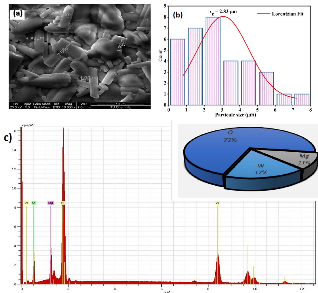
Fig. 3 (a) Scanning electron microscopy images, (b) distribution histogram of grains. (c) EDX spectrum of the compound LMWO.
