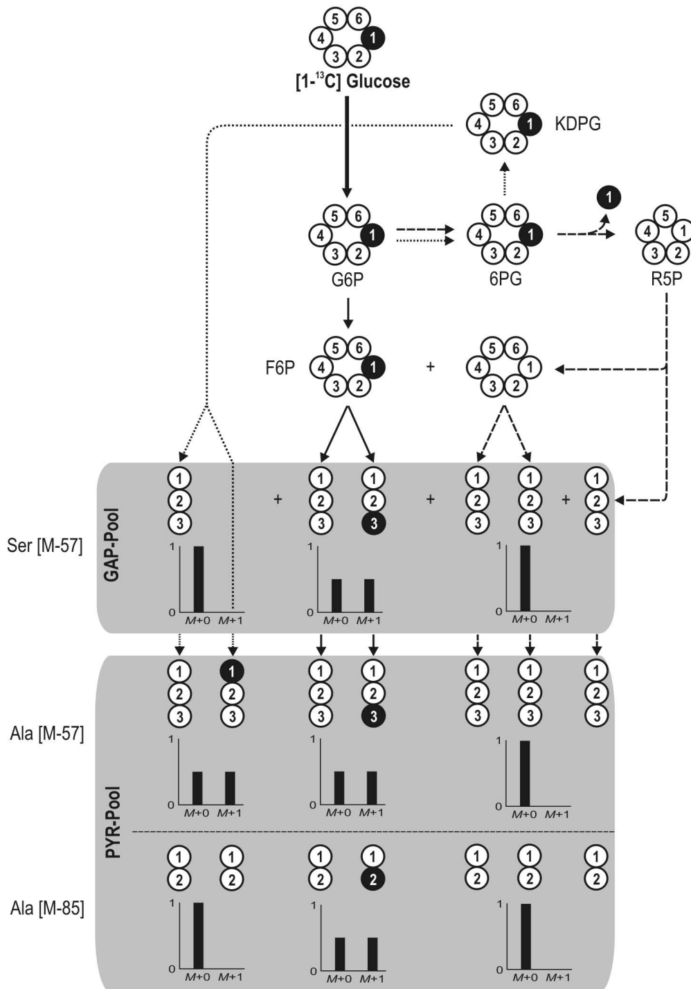
Figure 3 Theoretical labelling pattern of the C 3 pool (GAP and PYR) derived from 99% [1-^{13}\text{C}] glucose depending on activities in the carbon core metabolism. The three major routes for glucose catabolism are presented: glycolysis (solid lines), the pentose phosphate pathway (dashed lines) and the Entner-Doudoroff pathway (dotted lines). White circles represent unlabelled ( ^{12}\text{C} ) carbon whereas black circles indicate labelled ( ^{13}\text{C} ) carbon. The numbers reflect the position of the carbon atom within the molecule. Ala: alanine; G6P: glucose 6-phosphate; 6PG: 6-phosphogluconate; KDPG: 2-keto-3-deoxy-6-phosphogluconate; F6P: fructose 6-phosphate; R5P: ribose 5-phosphate; GAP: glyceraldehyde 3-phosphate; PYR: pyruvate.
