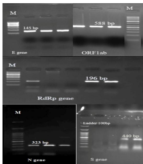
Fig. 2. Gel electrophoresis of five products in 2% gel agarose, M: Marker 100 bp E gene; 145 bp, ORF1ab: 588 bp, RdRp: 196 bp, N gene: 323 bp, S gene: 440 bp
