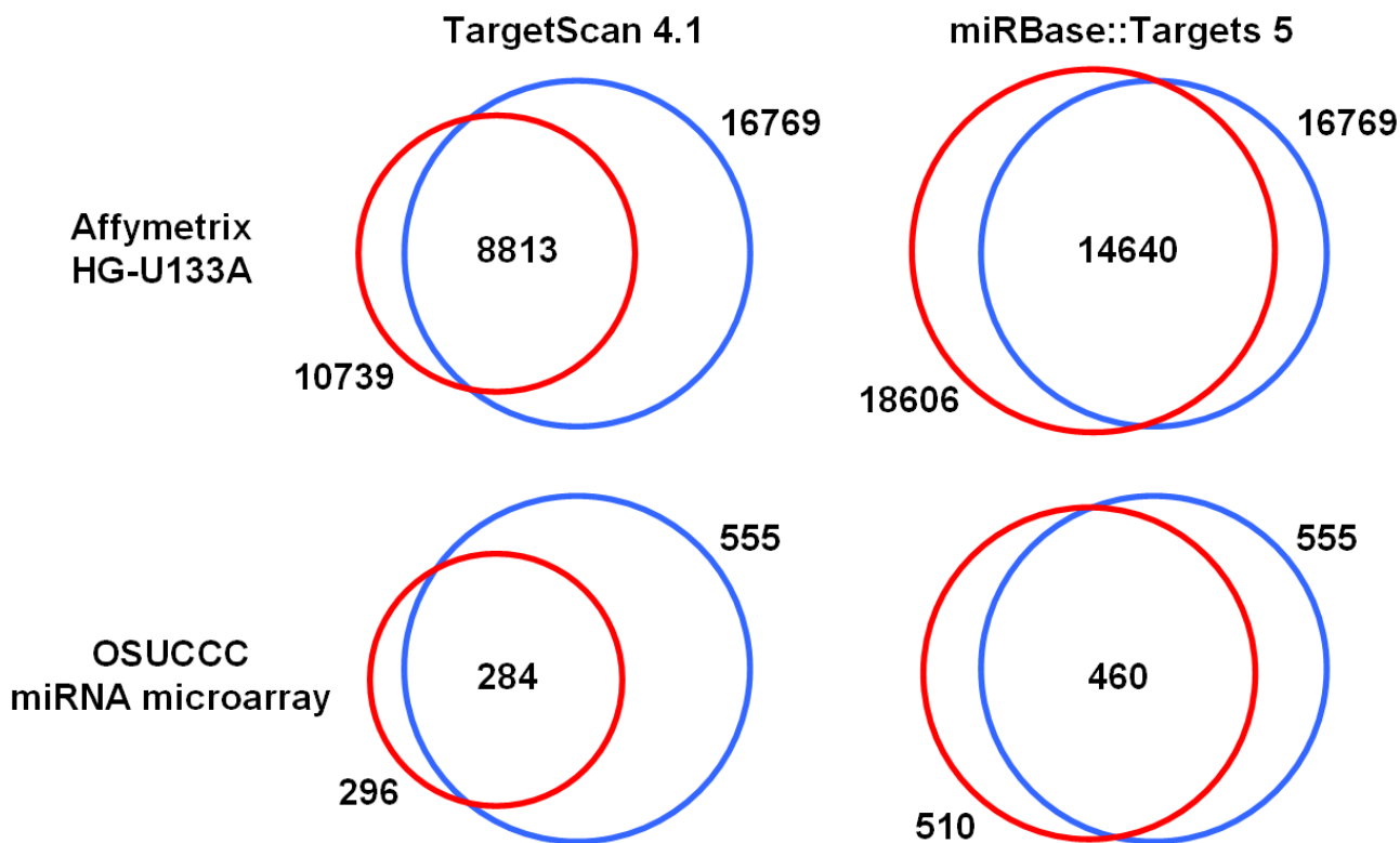
Figure 1 The number of microarray probes used for computing the correlations of expression profiles. The red circles denote the number of probes found in the predicted miRNA-target pairs. Two predicted data sources were used, including TargetScan 4.1 and miRBase::Target 5. The blue circles indicate the number of probes with at least two-fold intensity difference between the maximum and the minimum values across the NCI-60 samples. The intersection of the red and the blue circles is the number of probes used for the correlation analysis.
