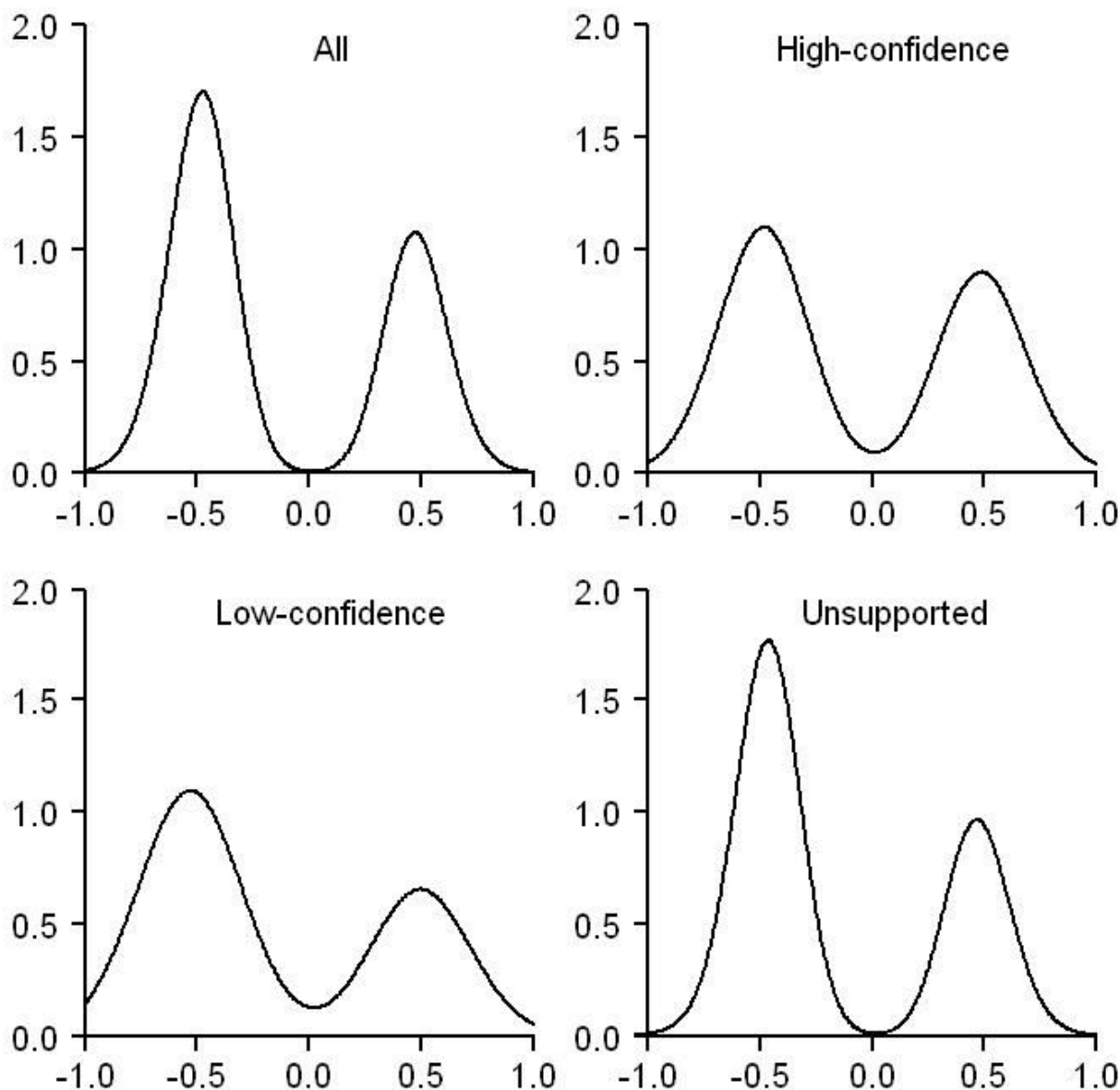
Figure 7 The density plot of the correlation coefficients computed using miRNA-mRNA pairs predicted by TargetScanS and then filtered by GenMiR++. The algorithm GenMiR++ provides a scoring system that determines the confidence level of the miRNA-mRNA interactions predicted by TargetScanS. There are three such levels: the high-confidence, the low-confidence and the unsupported. Using NCI-60 data, the distributions of Pearson correlation coefficients for the four categories specified by GenMiR++ (all, high-confidence, low-confidence and unsupported) are shown here. Only those correlations presenting Benjamini/Hochberg-corrected p -values < 0.05 are included. There are 412 such correlations in "All", 80 in "High-confidence", 41 in "Low-confidence" and 291 in "Unsupported".
