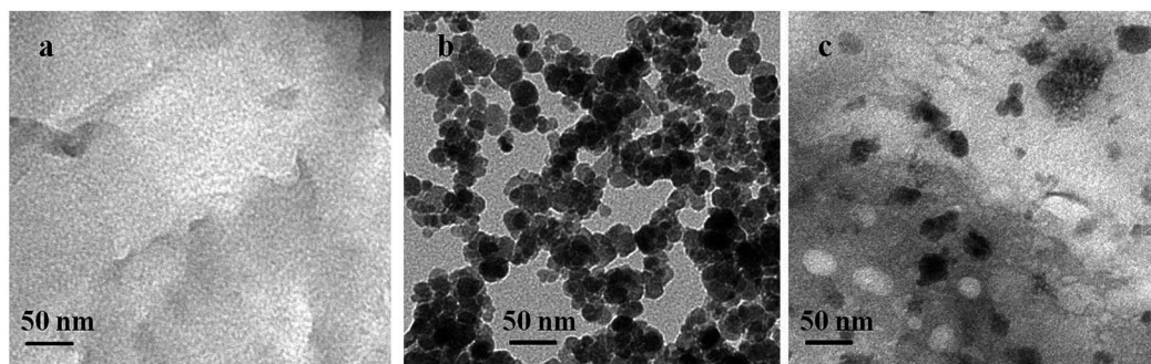
Fig. 1 TEM images of (a) pure g\text{-C}_3\text{N}_4 ; (b) pure \text{Fe}_3\text{O}_4 ; (c) \text{FeOCN-4} .
