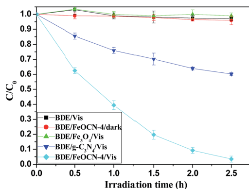
Fig. 6 Temporal curves of the degradation of BDE209 under different conditions. BDE209: 1.0 \times 10^{-5} mol L ^{-1} , FeOCN-4: 1 mg mL ^{-1} , solvent: CH _3 OH, wavelength > 420 nm, anoxic condition.
