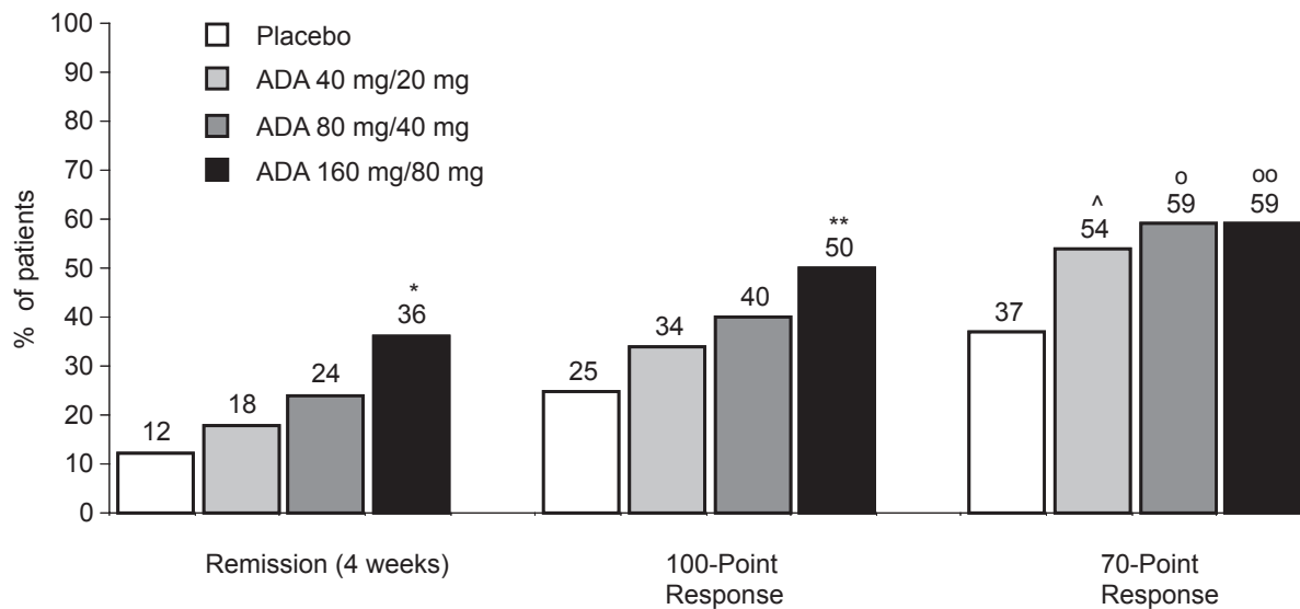
Figure 1 Efficacy of adalimumab (ADA) as induction therapy in CLASSIC I trial for Crohn's disease. Derived from Hanauer et al (2006). * p = 0.001 ; ** p = 0.002 ; ^ p < 0.05 ; ° p = 0.01 ; °° p = 0.007 .
