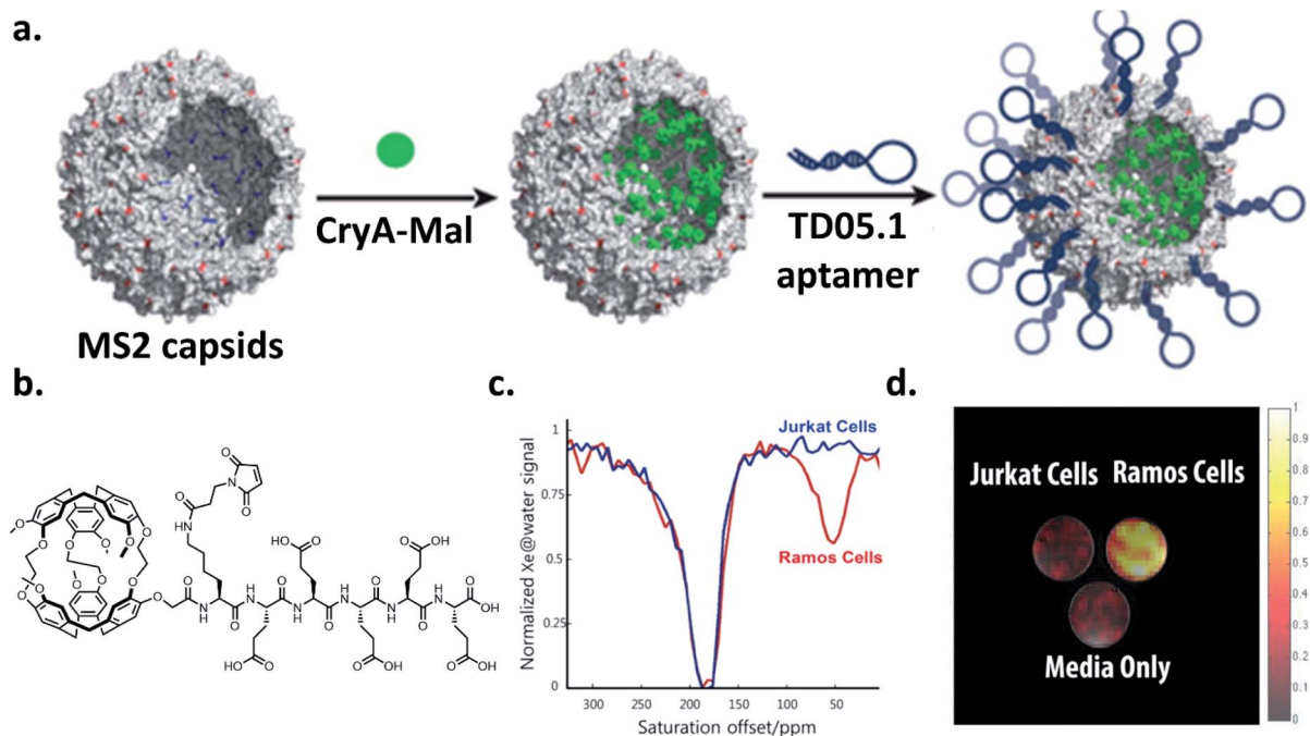
Fig. 7 (a) Scheme of bacteriophage–cryptophane biosensor assembly. The capsid interior of bacteriophage MS2 was modified with cryptophane-A conjugated to maleimide and five glutamic acids to increase solubility (CryA-Mal, green circle) at ca. 110 N87C positions. The capsid exterior was modified with 54 units of the TD05.1 DNA aptamer for targeting mIgM markers on lymphoma cells. (b) Chemical structure of CryA-Mal. (c) ^{129}\text{Xe} hyper-CEST NMR z-spectra of the biosensor (167 nM in capsids) incubated with 2 \times 10^7 Ramos (mIgM ^+ ) or Jurkat (mIgM ^- ) cells. (d) ^{129}\text{Xe} hyper-CEST MRI superimposed on ^1\text{H} MR image of tubes containing cell media only, and the two cell lines incubated with biosensor. Reproduced with permission from ref. 98. Copyright 2016 American Chemical Society.
