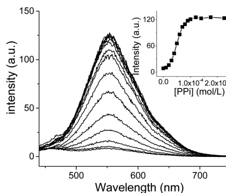
Fig. 2 The fluorescence change of 1 (50 μM) in water containing 50% DMSO with PPI in the presence of 1 equivalent zinc(II). Inset, curve of the intensity at 550 nm vs. the concentration of PPI. \lambda_{\text{ex}} = 378 nm, ex/em slits = 5/5 nm.
