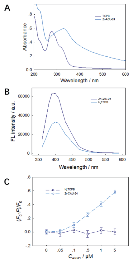
Fig. 4 UV-visible spectrum (A) and emission spectra ( \lambda_{em} = 410 nm) (B) of TCPB 4+ molecules and Zr-CAU-24 crystals. FL intensity fading of Zr-CAU-24 crystals and TCPB 4+ molecules with the existence of AFB1 (C).
