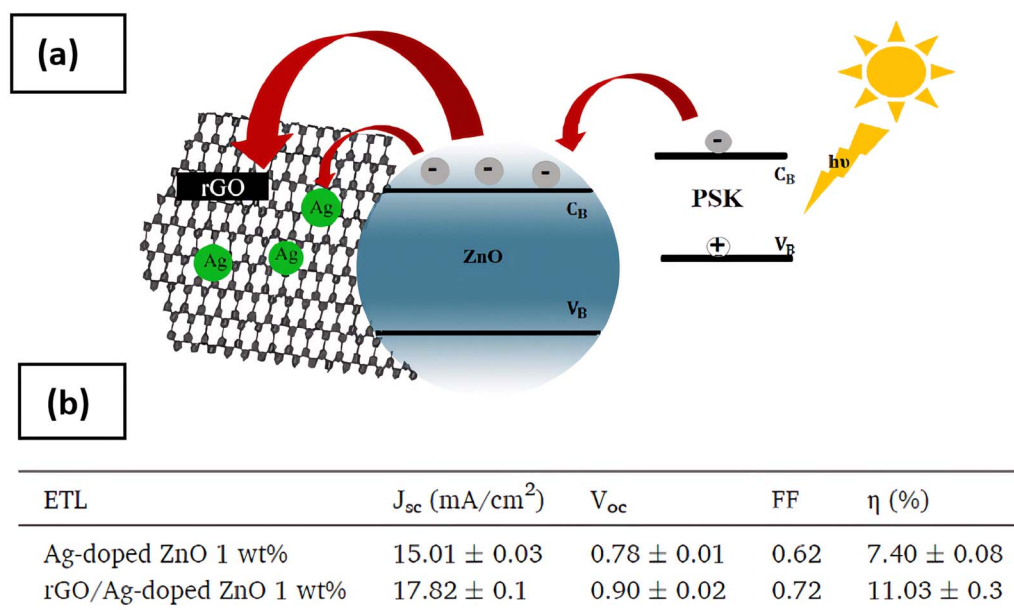
Fig. 20 (a) The functionality of rGO/Ag-doped (1 wt%) bilayer ETL of PSC ZnO. (b) J-V characteristics of Ag-doped and rGO/Ag-doped ZnO (1 wt%). Reproduced with permission from ref. 124. Copyright 2021 Elsevier.
