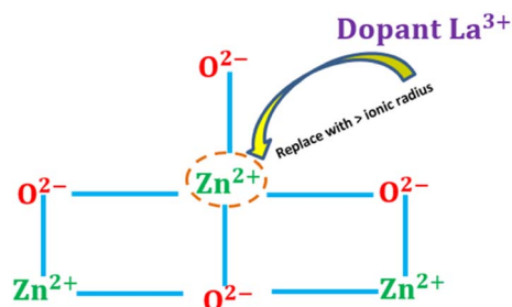
Fig. 18 A schematic image of the ZnO 2+ cation substitution or passivation in the doping engineering process with lanthanum as an additive dopant.
