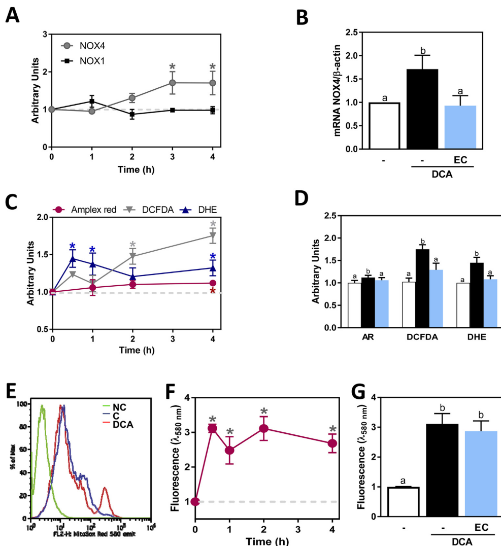
Fig. 3. DCA causes an increase in Caco-2 cell oxidant: effects of EC. Caco-2 cell monolayers were treated with 100 \mu M DCA in the absence or the presence of 5 \mu M EC for 0–4 h. A,B - mRNA levels of NOX1 and NOX4 were measured by RT-PCR and referred to \beta -actin mRNA content. mRNA levels were measured A -between 0–4 h for cells incubated without or with DCA, or B -for 2 h without or with addition of DCA and in the absence or the presence of 5 \mu M EC. C - Kinetics (0–4 h) of oxidant production evaluated using the probes Amplex ® Red (red circles), DCFDA (grey triangles), and DHE (blue triangles) as described in methods. D - Effects of DCA and 5 \mu M EC on oxidant production as measured with Amplex ® Red (AR) after 1 h incubation, or with DCFDA and DHE after 4 h incubation. E-G - Mitochondrial oxidant production was evaluated with MitoSOX. E - typical FACS scan profiles for cells incubated in the absence (C) or the presence of 100 \mu M DCA (DCA). NC: negative control of cells not added with MitoSOX. F - Kinetics of MitoSOX fluorescence of cells incubated in the presence of DCA. G - MitoSOX fluorescence in cells incubated without or with DCA and in the absence or presence of 5 \mu M EC for 2 h. Results are shown as mean \pm SEM of 4–5 independent experiments. Data were normalized to control values. Kinetic graphs: control values are shown as a dashed grey line. *Significantly different from controls at the corresponding time point. Bars: values having different superscripts are significantly different ( p < 0.05 , One-way ANOVA). (For interpretation of the references to color in this figure legend, the reader is referred to the Web version of this article.)
