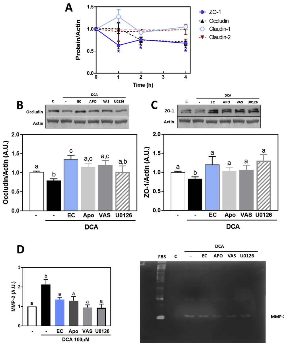
Fig. 6. DCA decreases the expression of tight junction proteins: effects of EC, NADPH oxidase and ERK1/2 inhibitors. Caco-2 cell monolayers were incubated for 0–4 h with or without 100 \mu M DCA and in the absence or the presence of 5 \mu M EC, 1 \mu M apocynin, 1 \mu M VAS-2870 or 10 \mu M U0126. The expression of TJ proteins (ZO-1, occludin, claudin-1 and claudin-2) was measured by Western blot. Bands were quantified and values referred to \beta -actin levels. A -Kinetics of DCA-mediated effects on ZO-1 (full circles), occludin (black triangles), claudin-1 (empty circles) and claudin-2 (red triangles) protein profiles. B -D- Effects of EC, apocynin, VAS-2870 and U0126 on occludin ( B ) and ZO-1 ( C ) protein levels and ( D ) MMP-2 activity measured by zymography after 2 h incubation with 100 \mu M DCA. Results are shown as mean \pm SE of 4–6 independent experiments. Values having different superscripts are significantly different ( p < 0.05 , One-way ANOVA test). (For interpretation of the references to color in this figure legend, the reader is referred to the Web version of this article.)
