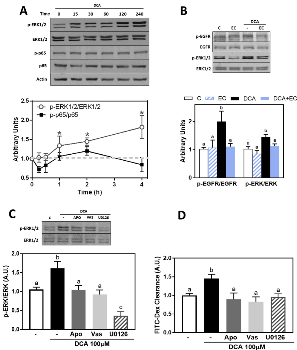
Fig. 4. ERK1/2 activation is involved in DCA-induced Caco-2 cell monolayer permeabilization: inhibitory actions of EC and other NADPH oxidase inhibitors. Caco-2 cell monolayers were incubated for 0–4 h with or without 100 μM DCA in the absence or the presence of 5 μM EC, 1 μM apocynin, 1 μM VAS-2870 or 10 μM U0126. A - The kinetics of ERK1/2 and NF-κB activation in the presence of 100 μM DCA was evaluated by Western blot by measuring the phosphorylation of ERK1/2 (T202/Y204) and p65 (Ser536), respectively. B - Cells were incubated with or without 100 μM DCA and in the absence or the presence of 1 μM EC for either 0.5 h to assess EGFR phosphorylation (Tyr1068) or 2 h for ERK1/2 phosphorylation. C , D - Cells were incubated with or without 100 μM DCA and in the absence or the presence of apocynin, VAS-2870 or U0126 for 2 h. C , D - Effects of the NADPH oxidase and ERK1/2 inhibitors on (C) DCA-induced ERK1/2 phosphorylation measured by Western blot, and (D) Caco-2 cell monolayer permeabilization evaluated as the FITC-dextran paracellular transport. Western blot bands were quantified and values for phosphorylated proteins were referred to the respective total protein content. Results are shown as mean ± SEM of 4–6 independent experiments. A - *Significantly different from controls at the corresponding time point. B - D - Values having different superscripts are significantly different ( p < 0.05 , One-way ANOVA).
