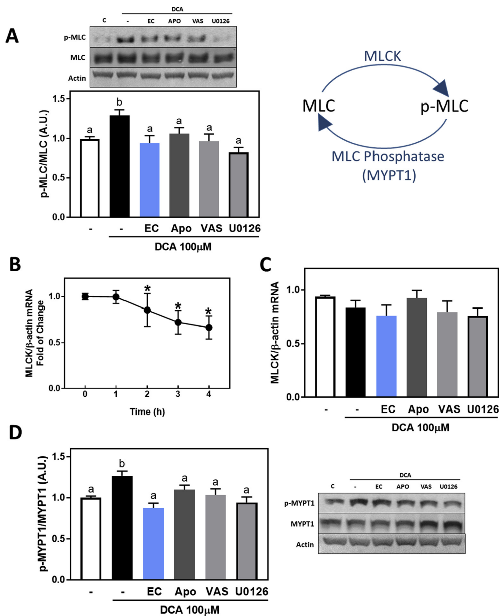
Fig. 5. DCA promotes an increase in MLC phosphorylation independently from MLCK but dependent on MLC phosphatase inhibition: effects of EC, and NADPH oxidase and ERK1/2 inhibitors. Caco-2 cell monolayers were incubated for 2 h with or without 100 μM DCA and in the absence or the presence of 5 μM EC, 1 μM apocynin, 1 μM VAS-2870 or 10 μM U0126. (A) MLC (Ser19) and (D) MYPT1 (Thr696) phosphorylation levels were measured by Western blot. After quantification values for phosphorylated proteins were referred to the respective total protein content. β-actin was measured as loading control. B,C-MLCK mRNA levels were measured by RT-PCR and values referred to the β-actin mRNA content. B- Kinetics of DCA-mediated effects on MLCK mRNA levels, C- Effects of the inhibitors on the MLCK mRNA content after 2 h incubation with DCA. Results are shown as mean ± SEM of 4–6 independent experiments. Values having different superscripts are significantly different (p < 0.05, One-way ANOVA).
