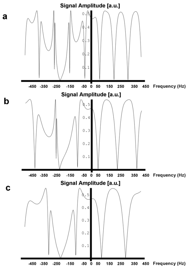
Figure 3 A comparison of simulated frequency response patterns for 1-(90°)-1 WE-SSFP with (a) TR = 8.9 ms (b) TR = 5.9 ms and (c) TR = 4.45 ms conditions. The fat frequency falls within the stopband in each case, indicating that fat suppression is independent of sequence TR.
