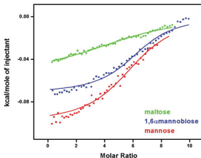
Fig. 3. Calorimetric titrations of griffithsin with mannose (red), 1,6- \alpha -mannobiose (blue) and maltose (green). The solid lines represent fits to the data. The overall \Delta H (kcal/mol) of binding are compared by superposition of all three isotherms.
