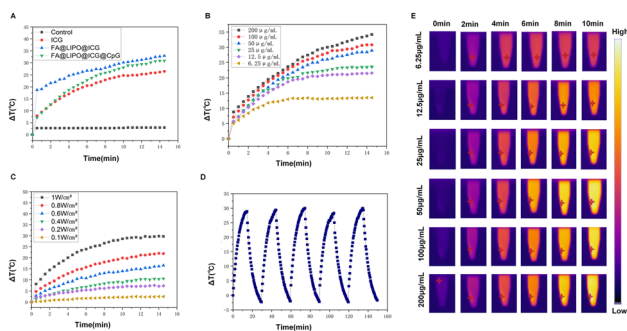
Fig. 2 In vitro photothermal experiments; (A) temperature increase in various solutions including water, ICG NPs, FA@LIPO@ICG NPs, and FA@LIPO@ICG@CpG NPs (calculated based on ICG content, ICG concentration at 200 \mu\text{g mL}^{-1} ) after 15 minutes of near-infrared laser irradiation; (B) temperature increase in FA@LIPO@ICG@CpG NP solutions of different concentrations after 15 minutes of near-infrared laser irradiation; (C) temperature increase in FA@LIPO@ICG@CpG NPs ( 200 \mu\text{g mL}^{-1} , calculated based on ICG content) under near-infrared laser irradiation with varying power densities for 15 minutes; (D) temperature changes in FA@LIPO@ICG@CpG NP water-dispersed solution ( 200 \mu\text{g mL}^{-1} , calculated based on ICG content) during 5 cycles of near-infrared laser irradiation/cooling. Excitation: 808 nm and power density: 1 \text{ W cm}^{-2} ; (E) infrared thermal images of FA@LIPO@ICG@CpG NP water-dispersed solution at different concentrations under near-infrared laser irradiation.
