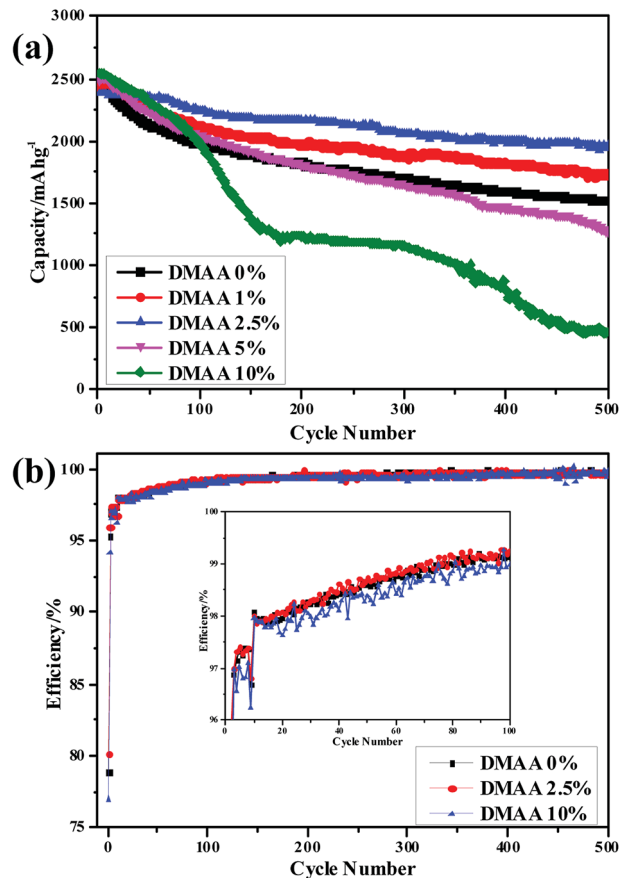
Fig. 6 (a) Cycling comparison and (b) coulombic efficiency of the silicon anode in 1 M \text{LiPF}_6/\text{EC} : \text{DMC} : \text{DEC} : \text{FEC} (3 : 3 : 3 : 1) electrolytes with different contents of DMAA additive.
