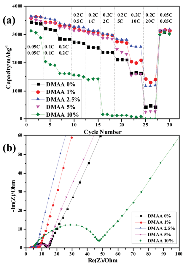
Fig. 5 (a) Rate capability and (b) Nyquist plots of the silicon electrode in 1 M \text{LiPF}_6/\text{EC} : \text{DMC} : \text{DEC} : \text{FEC} (3 : 3 : 3 : 1) electrolytes with different contents of DMAA additive.
