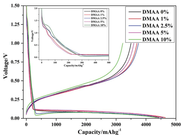
Fig. 4 Charge–discharge profiles for first cycle of the Si anode in 1 M \text{LiPF}_6/\text{EC} : \text{DMC} : \text{DEC} : \text{FEC} (3 : 3 : 3 : 1) electrolytes with different contents of DMAA additive.
