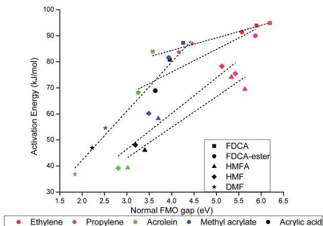
Fig. 6 Activation energy ( \text{kJ mol}^{-1} ) versus normal FMO gap (eV) for DA reaction of the molecules included in our scope of study.
