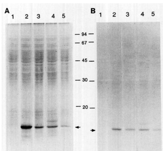
Fig. 5. Translation of MHV leader-human \alpha -globin chimeric mRNAs. Translation conditions employed were as described; 250 ng of each synthetic mRNA was used in the translation mixture (16.7 \mu g/ml final concentration) and incubation was at 37° for 60 min. Translation products were analyzed as described above. The autoradiogram is shown. Numbers in the center of the figure indicate positions of molecular size standards as described in the legend to Fig. 3. Numbers in parentheses after each mRNA represent relative expression of \alpha -globin with respect to h \alpha G mRNA control (lane 5) which was arbitrarily set to 1.0 in each panel. (A) Translation in infected DBT cell-free extract. Lane 1, no mRNA; lane 2, h \alpha GL1 (12.3); lane 3, h \alpha GL \Delta 62-74 (3.8); lane 4, h \alpha GL12 (3.6); lane 5, h \alpha G mRNA (1.0). (B) Translation in uninfected DBT cell-free extract. Lane 1, no mRNA; lane 2, h \alpha GL1 (3.3); lane 3, h \alpha GL \Delta 62-74 (1.4); lane 4, h \alpha GL12 (2.9); lane 5, h \alpha G mRNA (1.0). The arrows indicate the migration positions of human \alpha -globin in each polyacrylamide gel.
