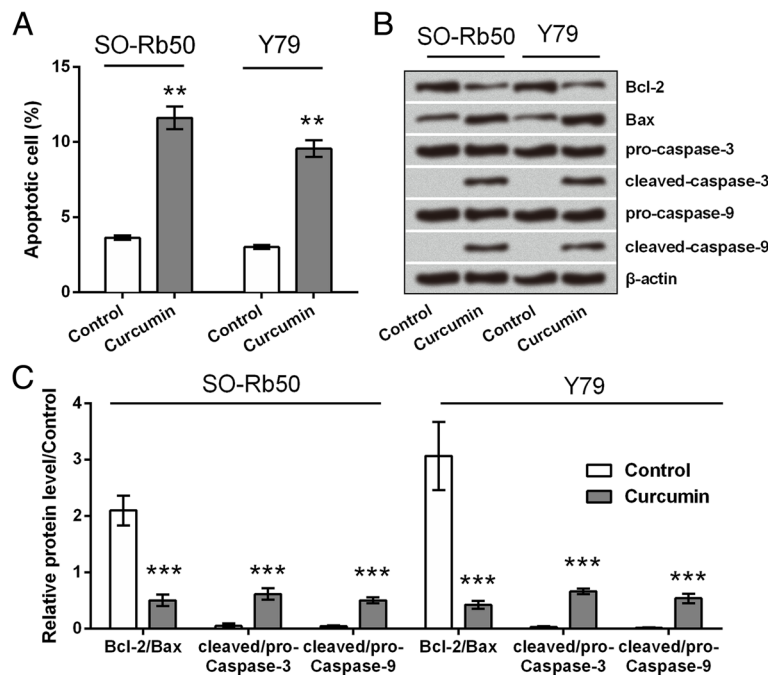
Fig. 2 Curcumin promoted apoptosis in SO-Rb50 and Y79 cells. a Apoptotic cell rate of cell pre-treated with 30 μM curcumin. b Protein expression levels of apoptosis-associated factors in cell pre-treated with 30 μM curcumin. c Quantitative protein levels. ** P < 0.01 , *** P < 0.001 vs. control group
