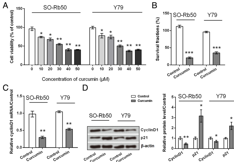
Fig. 1 Curcumin inhibited SO-Rb50 and Y79 cells proliferation. a Viability of cell pre-treated with 0–50 μM curcumin. b Colony formation capacity of cell pre-treated with 30 μM curcumin. c mRNA level expression of CyclinD1 in cell pre-treated with 30 μM curcumin. d Protein level expression of CyclinD1 and p21 in cell pre-treated with 30 μM curcumin. * P < 0.05 , ** P < 0.01 , *** P < 0.001 vs. control group
