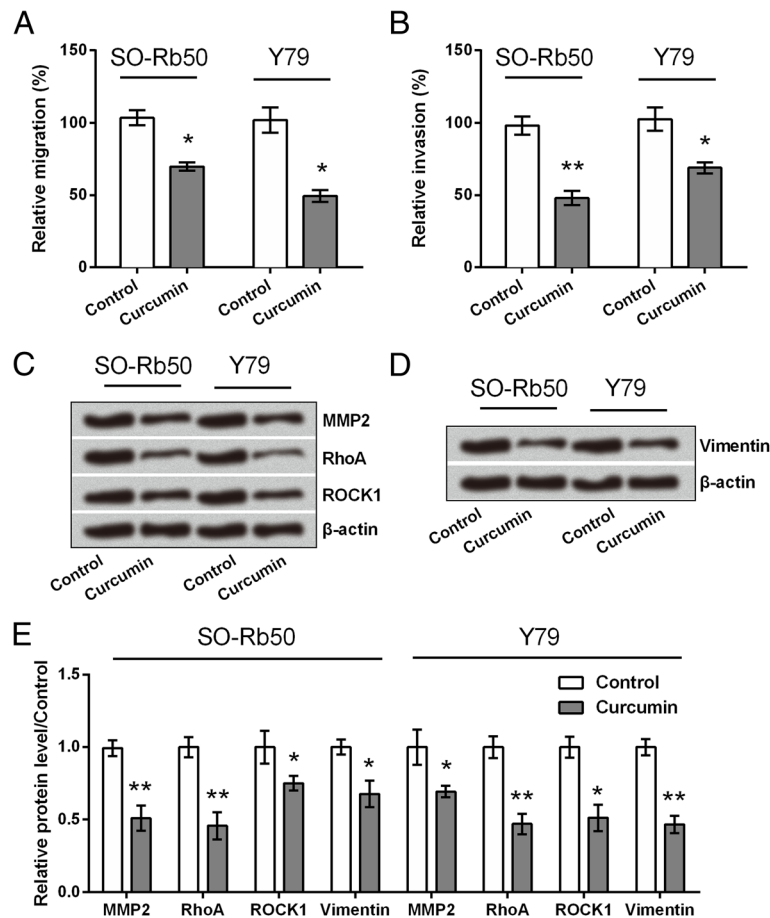
Fig. 3 Curcumin inhibited the migratory and invasive capacities of SO-Rb50 and Y79 cells. a Relative migration and (b) relative invasion of cell after treatment with 30 \mu M curcumin. c and d Protein expression levels of metastasis-related factors in cell pre-treated with 30 \mu M curcumin. e Quantitative protein levels. * P < 0.05 , ** P < 0.01 vs. control group
