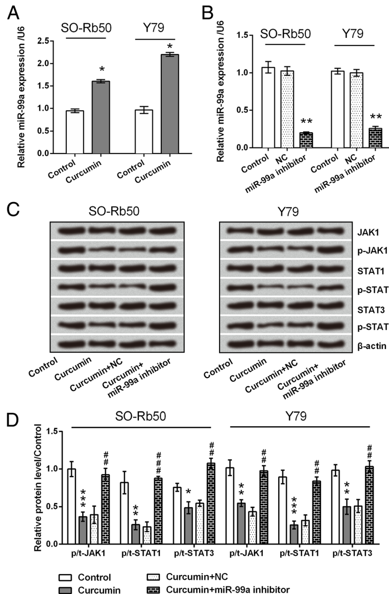
Fig. 4 Curcumin deactivated JAK/STAT signaling pathway. a miR-99a expression in cell pre-treated with 30 μM curcumin. b miR-99a expression in cell transfected with miR-99a inhibitor and NC. U6 snRNA was used as an internal control. c Protein expression levels of main factors in JAK/STAT pathway, after treatment with curcumin with or without miR-99a inhibitor transfection. d Quantitative protein levels. * P < 0.05 , ** P < 0.01 , *** P < 0.001 vs. control or NC groups. ## P < 0.01 , ### P < 0.001 vs. curcumin + NC group
