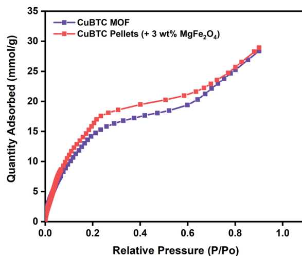
Fig. 2 Water vapour adsorption isotherms of CuBTC MOF and 3 wt% CuBTC–MgFe 2 O 4 composite pellets measured at 298 K.
