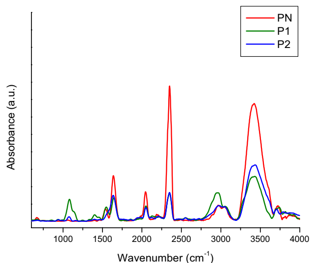
Figure 6. ATR-FTIR spectra of CRP standard (red), sample P1 (green), sample P2 (blue).
