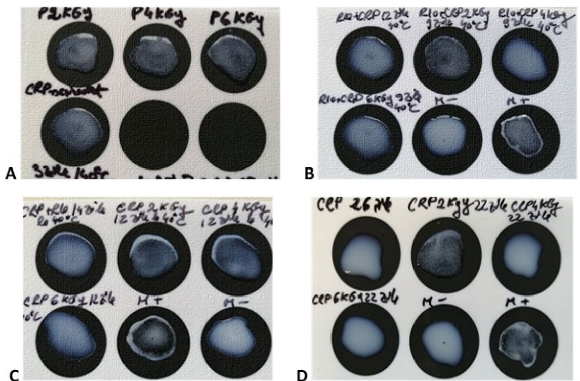
Figure 4. Agglutination results at different testing intervals: (A) after 3 days incubation at 40 °C; (B) after 9 days incubation at 40 °C; (C) after 12 days incubation at 40 °C; (D) after 22 days incubation at 40 °C.
