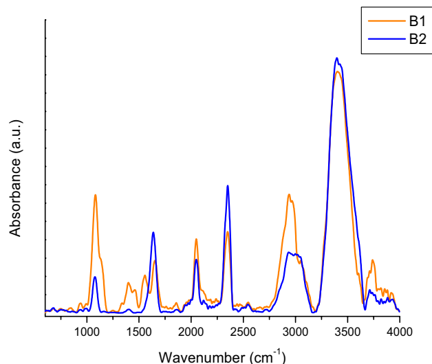
Figure 5. ATR-FTIR spectra for blank 1 (orange) and blank 2 (blue).
