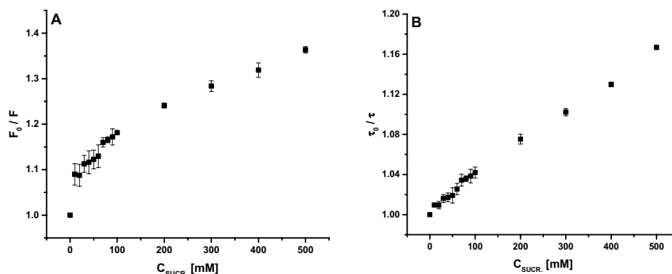
Figure 11. Stern–Volmer plots of CRP in presence of increasing concentrations of sucrose: steady state fluorescence (A) and fluorescence lifetime (B).
