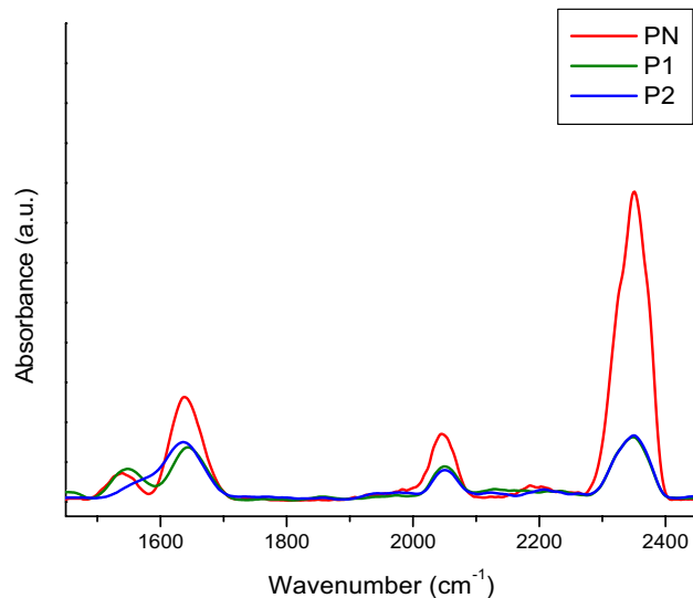
Figure 7. ATR-FTIR spectra of CRP standard (red), sample P1 (green), Sample P2 (blue), range from 1450 to 2450 \text{cm}^{-1} .
