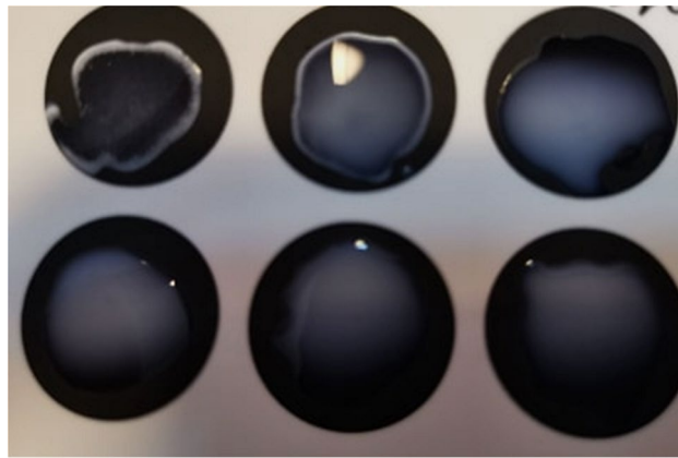
Figure 3. Agglutination reaction obtained using the LATEX-CRP detection kit at initial testing (T0).
