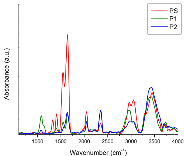
Figure 8. ATR-FTIR spectra for the Spinreact control (red), sample P1 (green) and sample P2 (blue).
