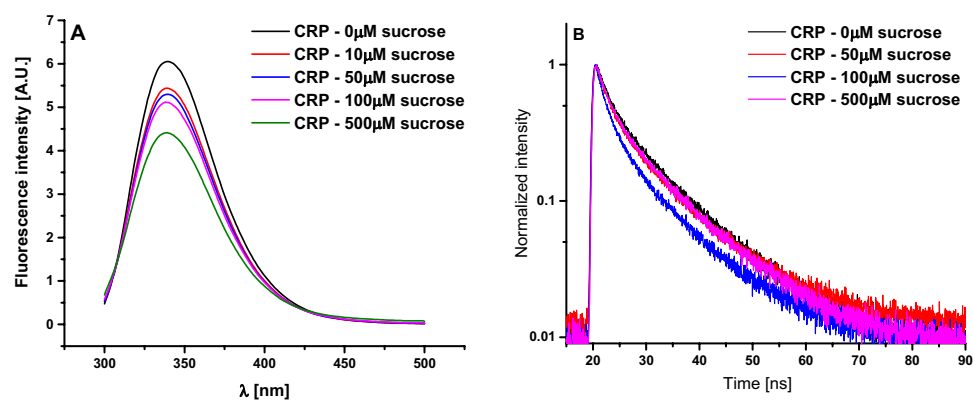
Figure 9. Fluorescence emission spectra for the sample containing CRP supplemented with different sucrose concentrations (A); Fluorescence lifetime spectra for the sample containing CRP supplemented with different sucrose concentrations (B).
