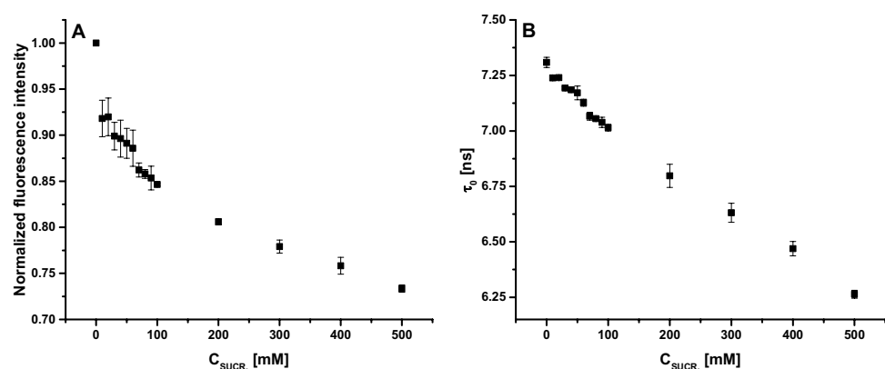
Figure 10. Normalized fluorescence intensity for peak maximum of emission spectra for the sample containing CRP supplemented with different sucrose concentrations (A); Fluorescence lifetime variation for the sample containing CRP supplemented with different sucrose concentrations (B).
