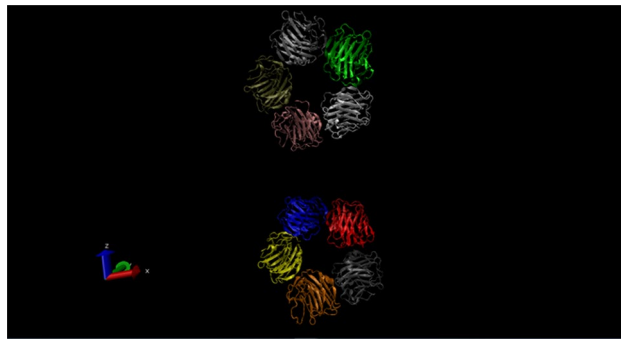
Figure 1. Pentameric structure of C-reactive protein obtained using the Visual Molecular Dynamics (VMD) software 2 .
