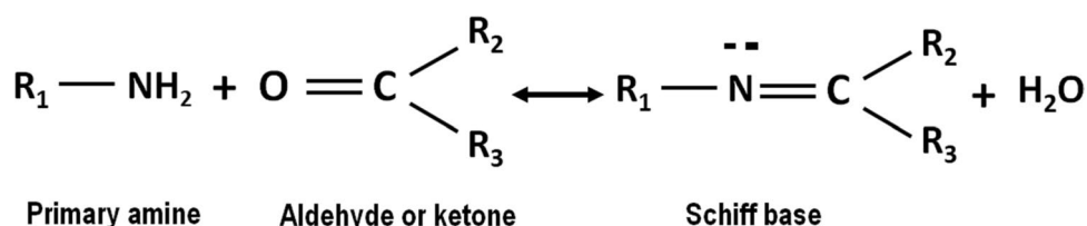
Figure 2. Schiff base formation.
