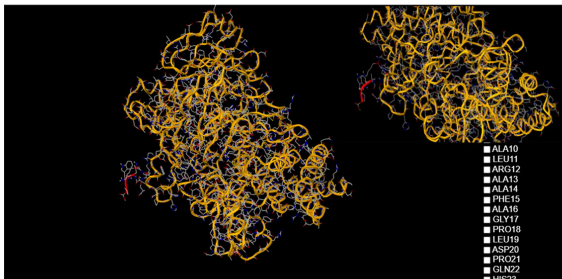
Figure 13. Result of the first docking experiment, with a score of -3.21 obtained using 1-CLICK DOCKING Software from the mcule platform, version from 2011, https://mcule.com/apps/1-click-docking/ .
