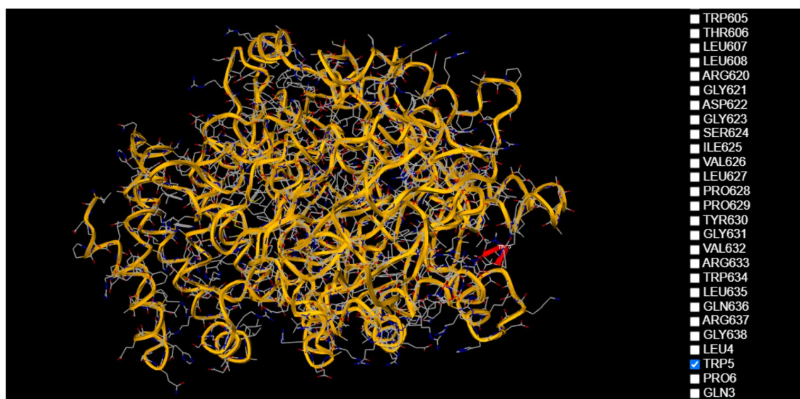
Figure 14. Bounding of the sucrose molecule near TRP5 obtained using 1-CLICK DOCKING Software from the mcule platform, version from 2011, https://mcule.com/apps/1-click-docking/ .
