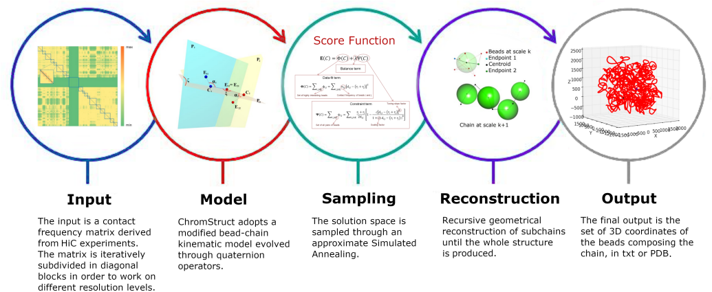
Figure 1. Flow of ChromStruct : (blue) the input HI-C contact frequency matrix is subdivided in diagonal blocks. (red) Chromatin fibre is modeled as a chain of partially penetrable beads and subdivided into sub-chains. (green) Geometrical perturbations are performed in the quaternion algebra and the solution space is sampled by a Bayesian method. (violet) As the last step, a multilevel 3D reconstruction generates chromatin output conformations (gray) that are compatible with input and constraints.
