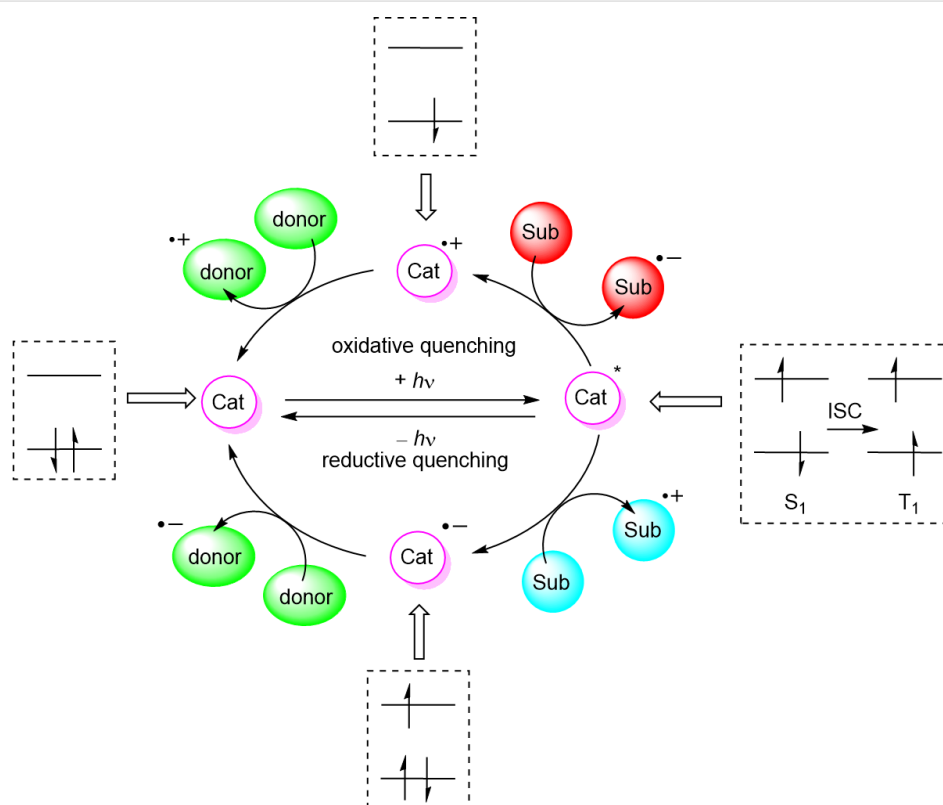
Scheme 4: Possible mechanisms of an immobilised molecular photoredox catalyst by oxidative or reductive quenching. ISC = intersystem crossing, Sub = substrate, Cat = photocatalyst, Cat* = electronic excited state photocatalyst, \pm h\nu = absorption/emission of photon, S_1 = first singlet electronic excited state, T_1 = first triplet electronic excited state.
