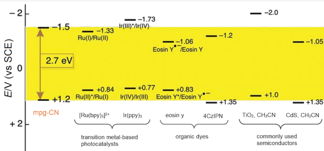
Figure 16: Electrochemical potential of common semiconductor, transition metal, and organic dye-based photocatalysts [128]. Reprinted with permission from AAAS.
