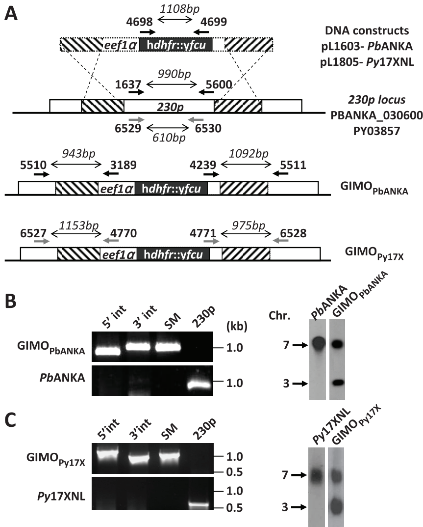
Figure 1. Generation and genotype analyses of P. berghei and P. yoelii GIMO mother lines. (A) Schematic representation of the constructs used to introduce the positive-negative selectable marker cassette in the P. berghei ( PbANKA ) or P. yoelii ( Py17XNL ) 230p locus. DNA constructs pL1603 (targeting P. berghei 230p, PBANKA_030600) and pL1805 (targeting P. yoelii 230p, PY03857) containing a fusion of the positive drug selectable marker dhfr (human dihydrofolate reductase) and negative marker yfcu (yeast cytosine deaminase and uridyl phosphoribosyl transferase) under the control of the eef1 \alpha promoter target the 230p locus at the target regions (hatched boxes) by double cross-over homologous recombination. Location of primers used for PCR analysis and sizes of PCR products are shown (see Table S2 for all primer sequences). (B) Diagnostic PCR and Southern analysis of PFG-separated chromosomes confirming correct integration of the construct in the P. berghei mother line GIMO PbANKA : 5' integration PCR (5' int; primers 5510/3189), 3' integration PCR (3' int; primers 4239/5511), amplification of dhfr::yfcu marker (SM; primers 4698/4699) and the original P. berghei 230p (230p; primers 1637/5600). Primer location (black arrows) and product sizes are shown in A. For Southern analysis, PFG-separated chromosomes were hybridized using a 3'UTR pbdhfr probe that recognizes the construct integrated into P. berghei 230p locus on chromosome 3 and the endogenous locus of dhfr/ts on chromosome 7. (C) Diagnostic PCR and Southern analysis of PFG-separated chromosomes confirming correct integration of the construct in the P. yoelii mother line GIMO Py17X : 5' integration PCR (primers 6527/4770), 3' integration PCR (primers 4771/6528), amplification of dhfr::yfcu marker (primers 4698/4699) and the P. yoelii 230p original locus (primers 6529/6530). Primer location (grey arrows) and product sizes are shown in A. For Southern analysis, chromosomal hybridization using a 3'UTR pbdhfr probe recognizes the construct integrated into P. yoelii 230p locus on chromosome 3 and the endogenous locus of dhfr/ts on chromosome 7. doi:10.1371/journal.pone.0029289.g001
