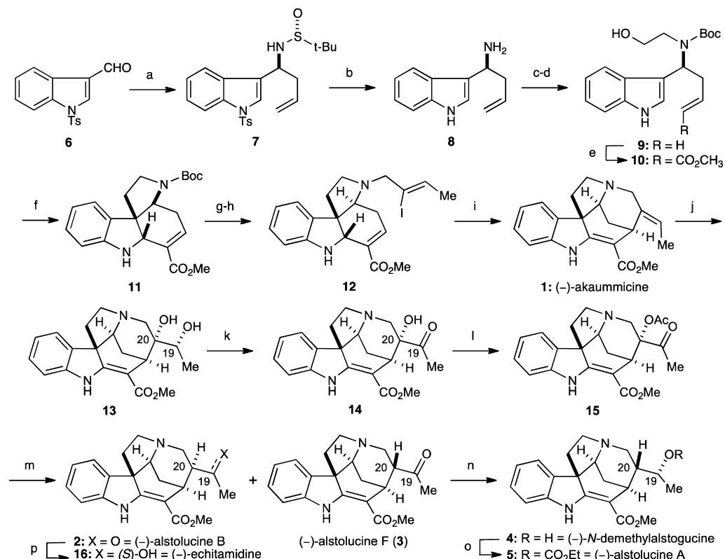
Scheme 1. Total Synthesis of (-)-Akuammicine (1), (-)-Alstolucine B (2), (-)-Alstolucine F (3), (-)- N -Demethylalstolucine (4), and (-)-Alstolucine A (5) a
