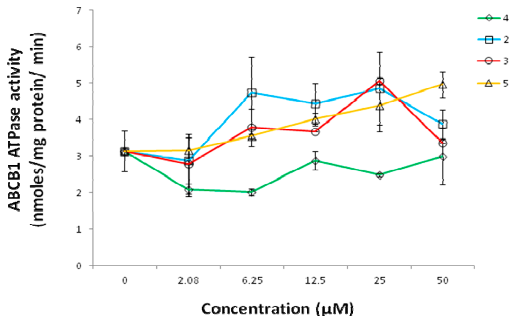
Figure 3. The effect of pentacyclic Strychnos alkaloids on ABCB1 ATPase activity. The ability of alstolucines and demethylalstogucine to inhibit ABCB1 ATPase activity was tested using a range of concentrations of alstolucine A (5), alstolucine B (2), alstolucine F (3), and N -demethylalstogucine (4). N -Demethylalstogucine (4) showed the only inhibition (~35–37%) at 2.08 and 6.25 \mu\text{M} , respectively. Experiments ( N = 3 ) were performed with duplicate samples.
