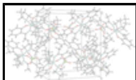
Fig. 2. The crystal packing of (I). The dashed lines denote hydrogen bonds.
