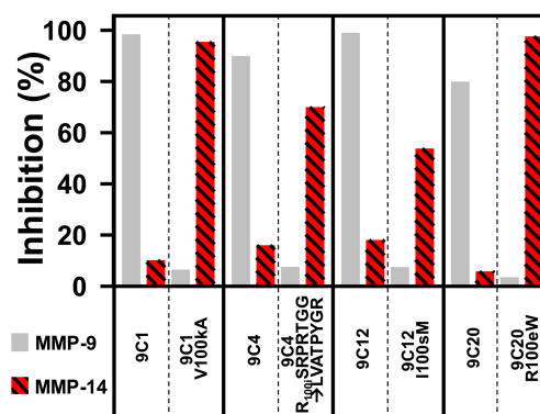
Figure 6. Paratope mutation studies of 9C1, 9C4, 9C12 and 9C20. The mutations in CDR-H3s were changed back to the amino acids of 3A2, and their inhibitory activities were tested. 500-nM scFvs and 10-nM cdMMP-9/-14 were used. Results were compared with inhibitory activities of 9C1, 9C4, 9C12 and 9C20 under the same assay conditions.
