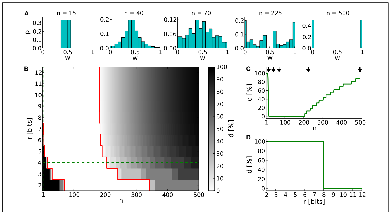
FIGURE 3 | The dynamic range for configurations of STDP on discrete weights. (A) Equilibrium weight distributions for a 4-bit weight resolution: Intermediate discrete weights partly project to themselves ( n = 15 ). The equilibrium weight distribution widens with an increasing number of SSPs ( n = 40 and 70 ). For a large number of SSPs ( n = 225 and 500 ) the intermediate discrete weights do not receive projections from others. (B) Percentage of dead discrete weights d . The limits of the
