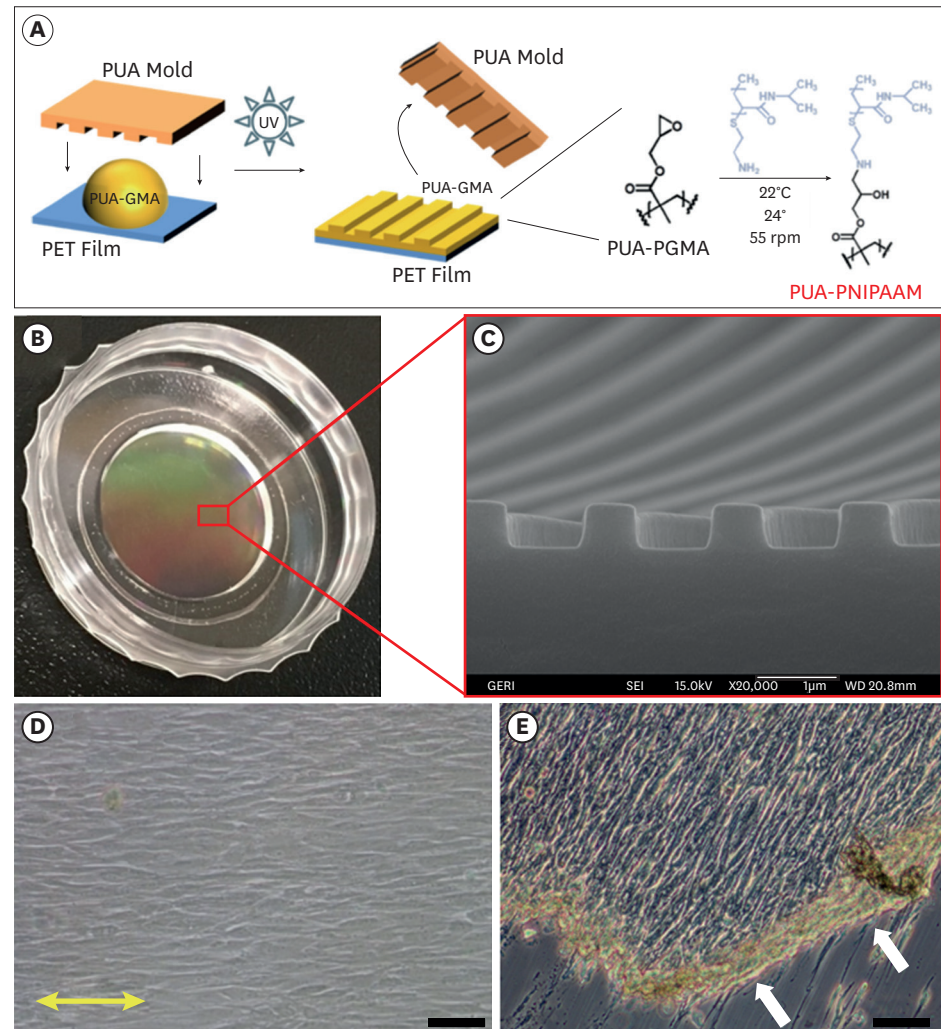
Figure 1. (A) The PNIPAM-functionalized thermoresponsive substratum with nanopatterns. Capillary force lithography was used for the fabrication of the substratum, with subsequent modification using amine-terminated PNIPAM on the PET film. (B) Representative macroscopic image of a large-area, scalable substratum, and (C) an SEM image of the 800-nm nanopatterned surface. (D) A microscopic view of hPDLSCs cultured on the 800-nm width nanopatterned surface incubated at 37°C for 48 hours following cell seeding. The yellow arrow designates the direction in which the hPDLSCs were aligned (scale bar=200 \mu\text{m} ). (E) Cell sheet detachment from the substratum after low-temperature treatment. An aligned and interconnected hPDLSC sheet with intact cell-to-cell junctions was slowly detached from the substratum as a single monolayer sheet upon water penetration from the periphery after being maintained at 22°C for 30 minutes. The white arrow indicates the direction of detachment (scale bar=200 \mu\text{m} ).
