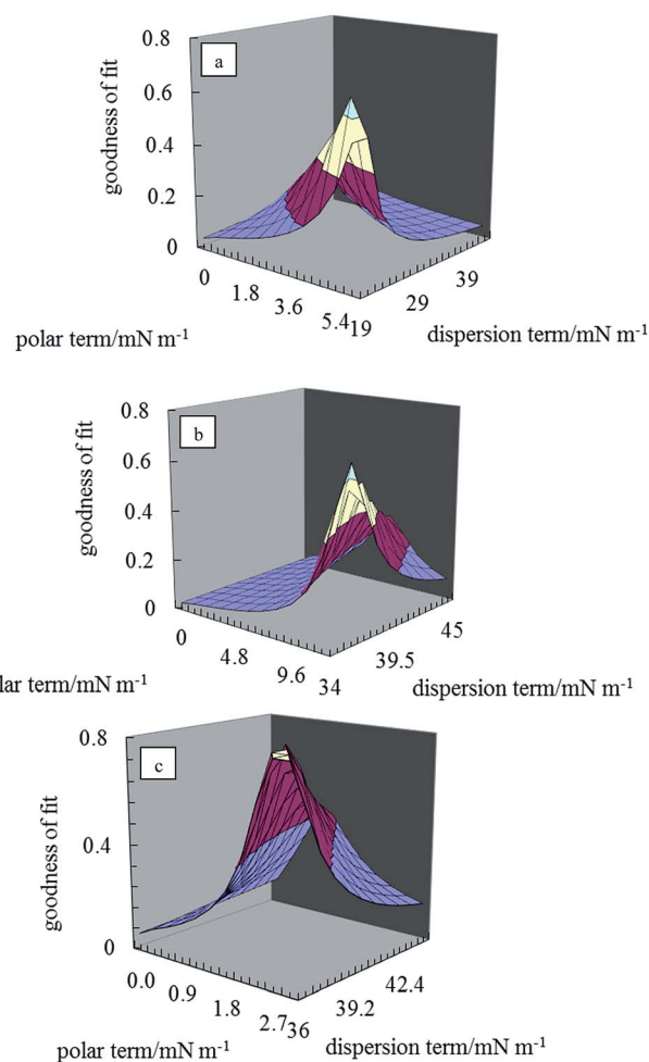
Fig. 2 3-D surface energy plots for disks of the pigment particles for different values of \gamma_{sa}^d and \gamma_{sa}^p for pigments (a) PR, (b) PO, (c) PV.
