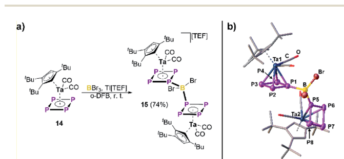
Fig. 4 (a) Reactivity of 14 towards the in situ formed dibromoboronium ion [BBr 2 ][TEF] + ; (b) molecular structure of 15 in the solid state (hydrogen atoms and the counter ion are omitted for clarity and thermal ellipsoids are drawn at the 50% probability level).
