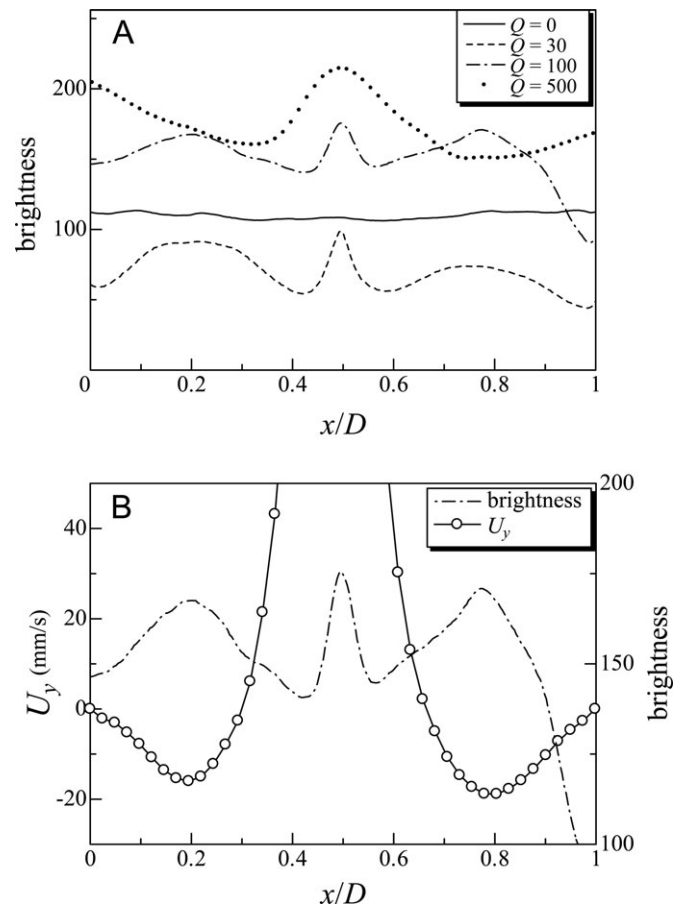
Fig. 5. Investigation into the mechanisms of vertical layer formation. (A) Effect of bubble flow rate Q on the brightness, and (B) changes in brightness and vertical velocity ( U_y ) when Q=100 \mu\text{l}/\text{min} , across a range of vertical velocity of background flow ( x/D ; where x indicates the horizontal direction of motile cells, cell concentration C=1 \times 10^6 cells/ml, diameter D=40 mm, with blue light). Brightness of time-averaged images is shown, indicating the cell distribution. The data is averaged in the depth direction from 35 to 70 mm from the top.
