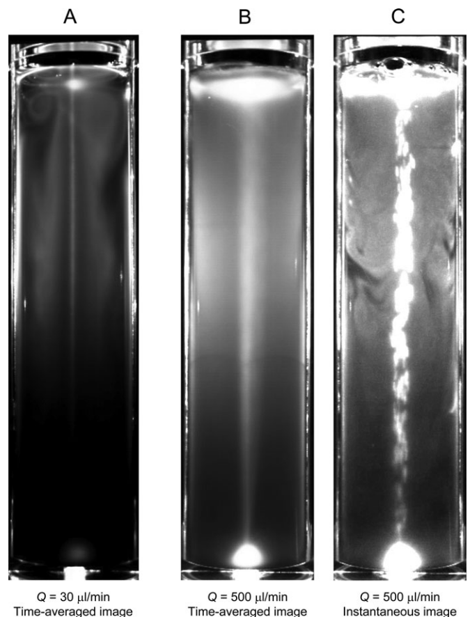
Fig. 3. Different bubble flow rates affect vertical distribution of motile cells. Effect of flow rate on the distribution of motile cells (wt), where Q is the bubble flow rate (cell concentration C=1\times 10^6 cells/ml, diameter D=40 mm, with blue light).
