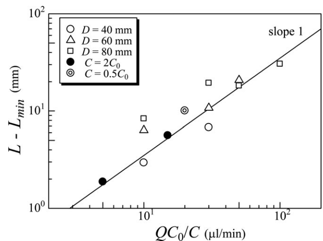
Fig. 9. The size of the vortical ring of cells is mainly a function of flow rate and cell density. Center-to-center distance L , smaller than D/2 , is plotted in log-log scale against QC_0/C for all experimental conditions (diameter D=40 , 60, and 80 mm; normalized cell concentration C/C_0=0.5 , 1, and 2, where C_0=1\times 10^6 cells/ml; with blue light). A fitted line of L-L_{\min}=0.35(QC_0/C) with r^2=0.85 and L_{\min}=15 mm (slope 1) is also drawn for comparison.
