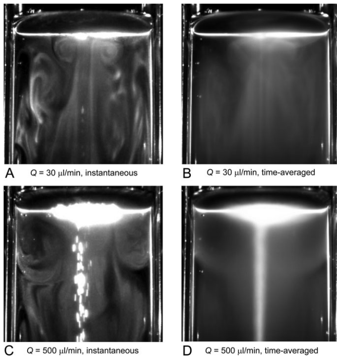
Fig. 6. Length scale of the vortical ring of cells increases with bubble flow rate. Distribution of motile cells (wt) in a container with diameter D=80 mm (cell concentration C=1\times 10^6 cells/ml, with blue light). Each figure shows instantaneous (A,C) or time-averaged (B,D) image of upper half of the container with bubble flow rate Q=30 \mu\text{l}/\text{min} (A,B) or 500 \mu\text{l}/\text{min} (C,D).
