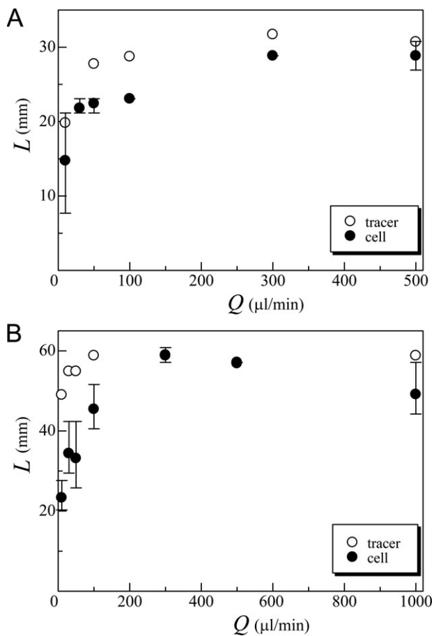
Fig. 8. Center-to-center distance ( L ) of the vortical ring of cells is smaller than that of the background flow, especially under low flow rate. Two kinds of containers with diameter D=40 mm (A) and D=80 mm (B) are examined across a range of bubble flow rates Q (cell concentration C=1\times 10^6 cells/ml, with blue light). The center-to-center distance L between the bubble flow (tracer) and the cell distribution (cell) shows that cells accumulate near the free surface then sediment relative to the surrounding fluid, which generated a downward motion earlier than in the background flow. Error bars indicate the maximum and minimum values
