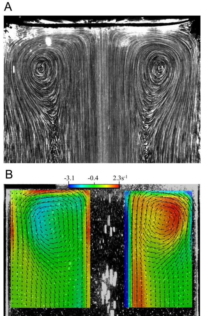
Fig. 7. Using tracer particles to investigate the background flow generated by bubbles. (A) The trajectories of tracer particles used to visualize the background flow generated by bubbles with bubble flow rate Q=100 ml/min, in the absence of cells. Upper region of the container is shown (diameter D=40 mm). (B) Velocity vectors and vorticity analysis of A, color indicates the vorticity.
