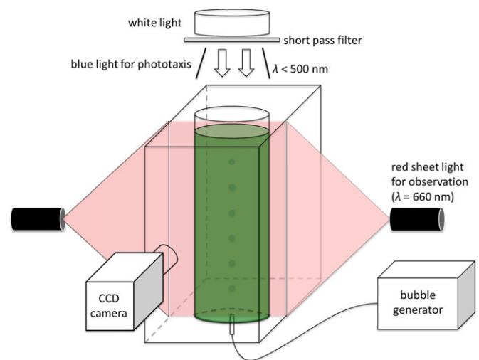
Fig. 10. Schematic of the experimental apparatus. A cylindrical container, made from a rectangular acrylic block, was filled with culture fluid. The container was illuminated from both sides by two laser sheets with a wavelength of 660 nm. When we explicitly observed phototactic responses by the cells, the container was illuminated by LED light from the top. Cell distribution was recorded with a CCD camera.
