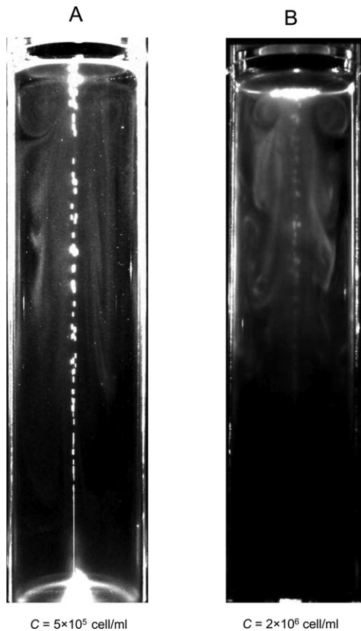
Fig. 4. Increased cell suspension density leads to a smaller vortical ring distribution. Instantaneous images showing that in a lower density of cells ( C=5 \times 10^5 cells/ml), vortical distribution near the free surface extends to the cylinder wall. However, in a higher density of cells ( C=2 \times 10^6 cells/ml), the vortical distribution did not reach the wall, indicating a smaller vortical ring (bubble flow rate Q=100 \mu\text{l}/\text{min} , diameter D=40 mm, with blue light).
