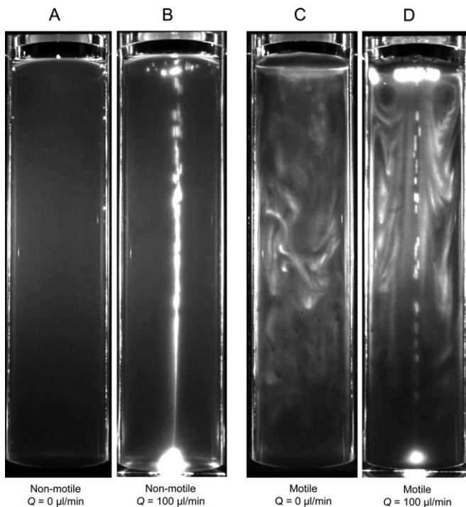
Fig. 1. Motility is required for inhomogeneous cell distribution in a bubble plume. Sample snapshots of non-motile ( pf14 ; A,B) and motile (wt; C,D) cell distribution with bubble flow rates of Q=0 \mu\text{l}/\text{min} (A,C) or Q=100 \mu\text{l}/\text{min} (B,D), after the suspension reached the equilibrium state (cell concentration C=1 \times 10^6 cells/ml, diameter D=40 mm, with blue light), showing that inhomogeneous distributions were only created by motile cells. Bubbles and cells are seen in white. The aspect ratio of the images was not modified throughout the paper.
