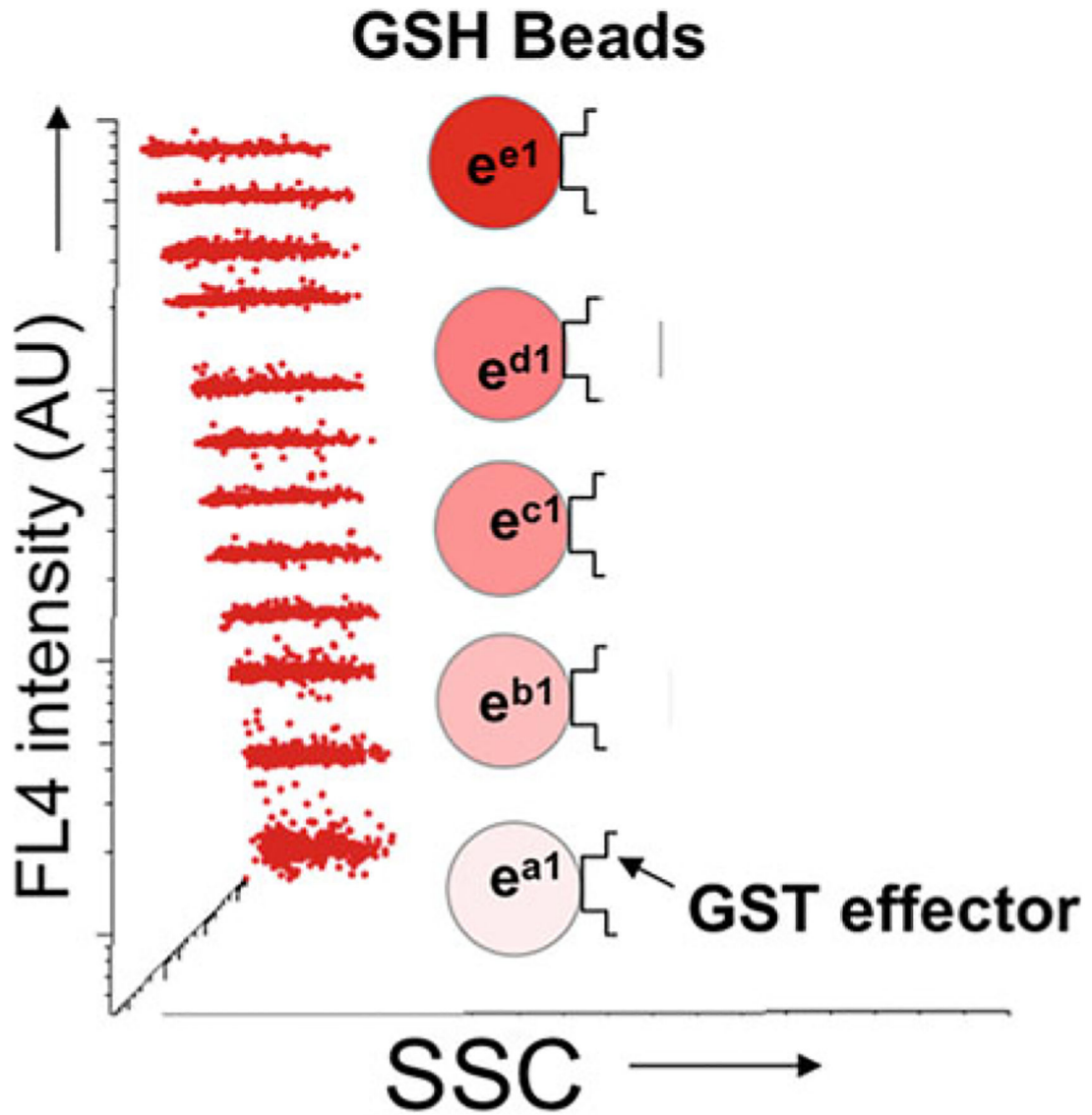
Fig. 1. The GTPase effector trap flow cytometry assay (G-Trap). The plot of red fluorescence (FL4) versus side scatter (SSC) of a set of 12 of Cyto-Plex™ beads dyed with 12 discrete levels of 700 nm fluorescence. In the G-Trap assay, the letters a , b , c , d , and e identify and link effectors, their cognate GTPases, and fluorescently labeled antibodies FL1 (520 nm emission) or FL2 (580 nm emission) used for readout. In single or multiplex format, glutathione bead populations coated with effectors are used to capture specific active GTPases. In multiplex format, the effector and GTPase identities are defined by the intensity level of red fluorescence encoded on each bead
