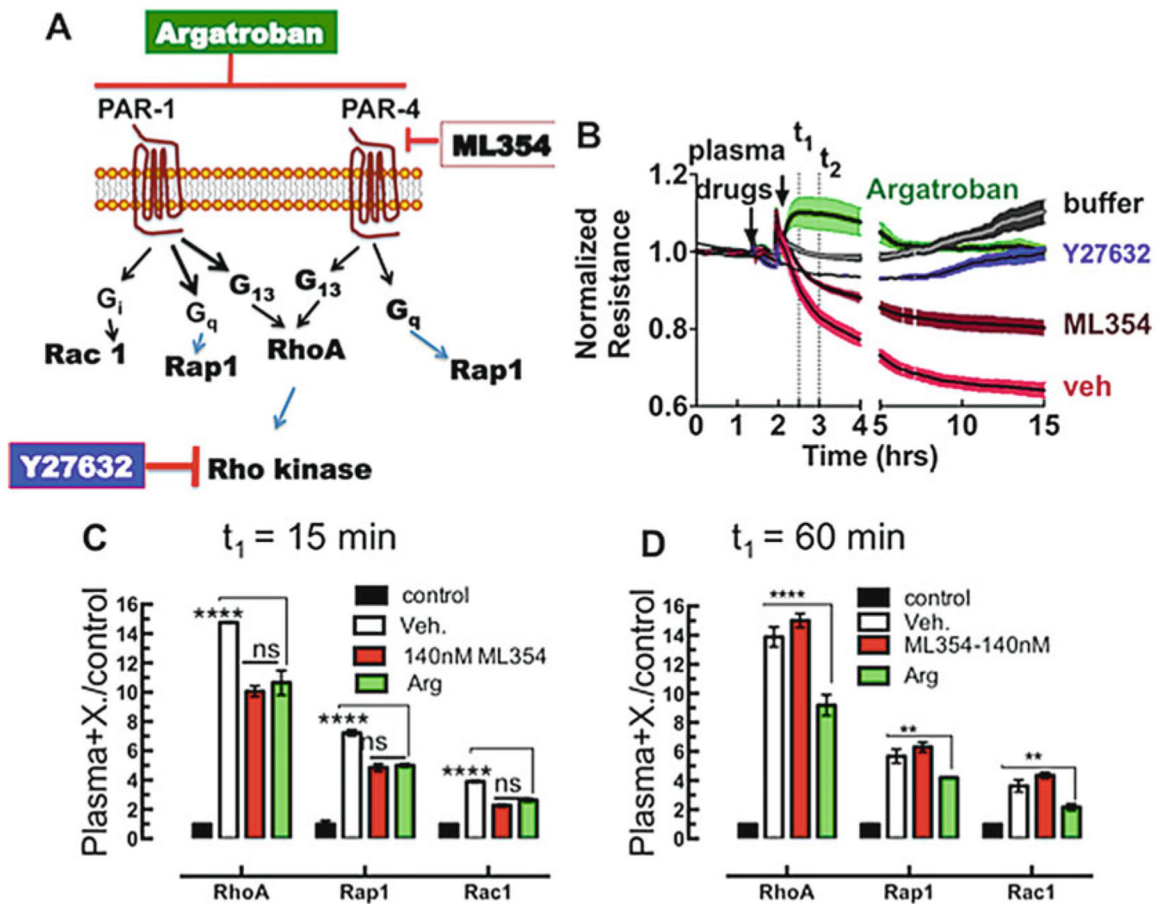
Fig. 4. RhoA activation stimulates loss of cell barrier function. (a) Model of protease-activated receptor-1 and -4 (PARs) coupling to multiple G proteins ( G_{\alpha_{i/o}} , G_{\alpha_q} , and G_{\alpha_{12/13}} ), upstream of small GTPase activation. Activation of PARs results in cell barrier disruption (RhoA) whereas Rac1 and Rap1 signaling are believed to be barrier protective [57–58]. Argatroban is an orthosteric inhibitor of thrombin interaction with PARs and is barrier protective. ML354 is a specific inhibitor of PAR4 activation. (b) Electric cell-substrate impedance sensing (ECIS) measurement of the effects of plasma from a patient with hantavirus cardiopulmonary syndrome (HCPS) on the cell barrier function of telomerase-immortalized microvascular endothelial (TIME) cell monolayers. Inhibitors are added to cell monolayers 30 min before the plasma is added as indicated by arrows and barrier function is measured. (c) GTPase activity measured in TIME cells after t_1 = 15 -min exposure to HCPS plasma. The results are corrected for nonspecific binding and normalized to resting cells. GTP loading increases in plasma treated cells. Drugs limit the increase in GTP loading compared to untreated cells. GTP loading in cells treated with ML354 is comparable to argatroban treatment. Cell barrier disruption is consistent with a significant increase in GTP loading in RhoA. Each multiplex data point was measured using effector beads prepared as described in Subheading 3.3. (d) After 1-h exposure to plasma, RhoA activity is observed in ML354 but not argatroban-treated samples. GTP loading is consistent with cell barrier disruption shown in the ECIS time course. The multiplex beads used for this dataset were
